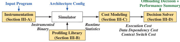
Fig. 4. PIMProf overview.
