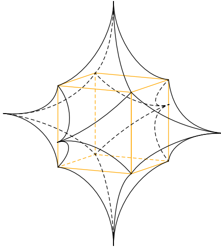
Figure 2: The polytope Q^3 .
