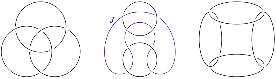
Figure 1: The links 6_2^3 , 8_9^3 and 8_2^4 .
