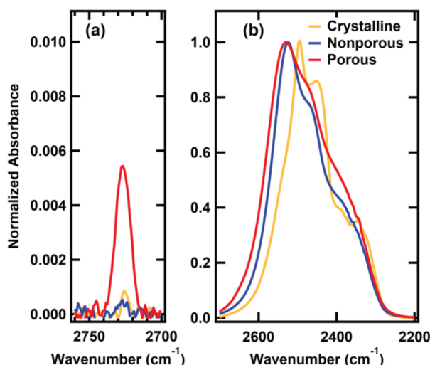
Figure 1. Normalized infrared spectra of 150 ML crystalline (CI, yellow), nonporous amorphous (np-ASW, blue), and porous amorphous (p-ASW, red) D_2O ices in the O–D stretch region between 2760 and 2700 cm^{-1} (a) and 2700 and 2200 (b) cm^{-1} dosed at 150, 108, and 20 K, respectively, and collected at 68 K. The region between 2760 and 2700 cm^{-1} (a) demonstrates that while dangling O–D are observed for all films, the intensity is greatest for the p-ASW films.
