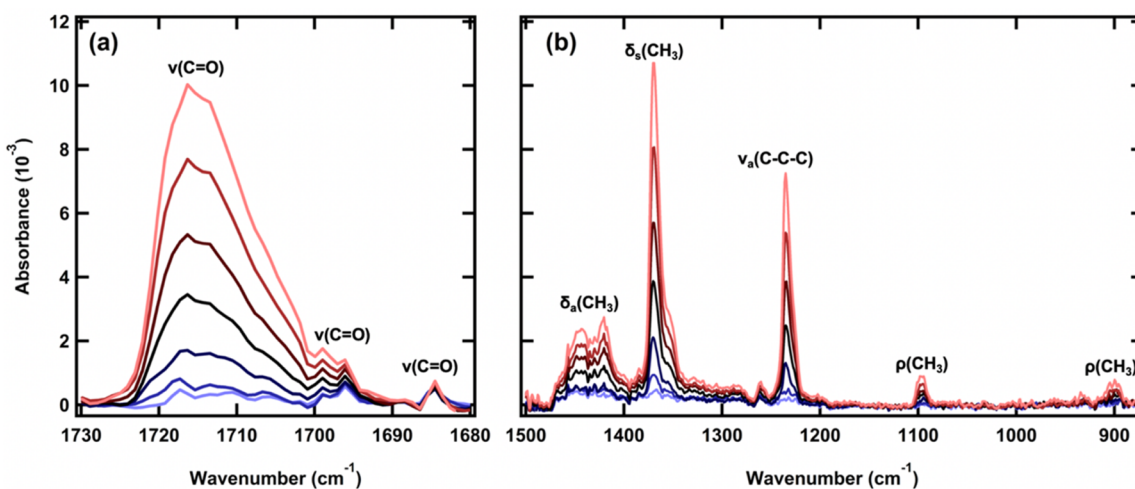
Figure 2. RAIR spectra of 1–24 ML of acetone adsorbed on Au(111) at 68 K. The RAIR spectra are separated into two wavenumber regimes: (a) C=O stretching between 1730 and 1680 cm^{-1} and (b) CH_3 deformation and rocking modes between 1500 and 875 cm^{-1} . The spectra correspond to 1, 1.7, 4.2, 8.3, 13, 19, and 24 ML of acetone.
