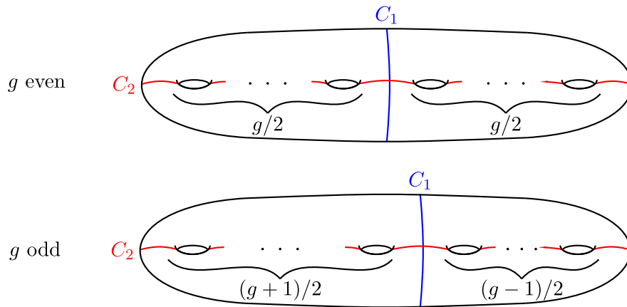
FIGURE 3. (Colour online) The dividing sets for Theorem 2.4.
