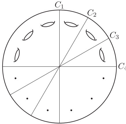
FIGURE 2. The separating curves in Theorem 2.3.
