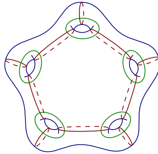
FIGURE 8. (Colour online) The two multicurves used in the proof of Theorem 1.5.
