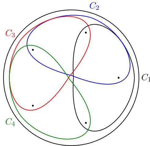
FIGURE 4. (Colour online) The curves in the proof of Theorem 2.5.
