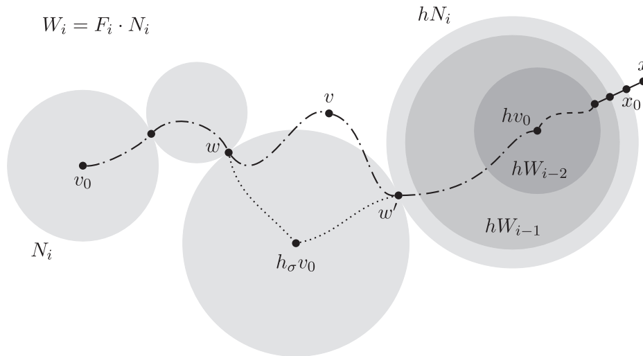
FIGURE 7. Steps 1 and 2 of statement (C) in the proof of Theorem 1.6.
