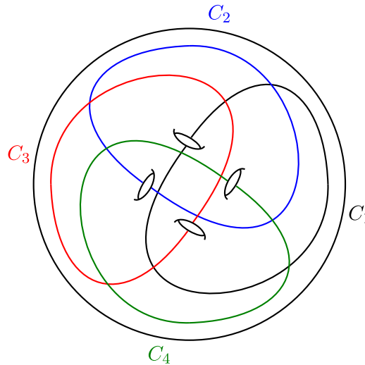
FIGURE 5. (Colour online) The curves in the proof of Theorem 2.6. Each C_i is symmetric about the plane of the page, and only half of each curve is shown.
