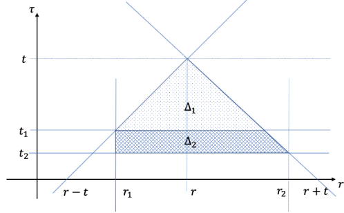
FIGURE 1. The domain \Delta
