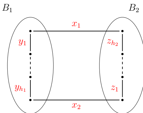
Figure 6: Cycle based on two edges between blocks.
