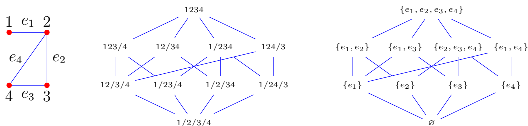
Figure 3: Figure for Example 1. On the left is the graph G , in the middle BL(G) in terms of vertices, and on the right BL(G) in terms of edges.
