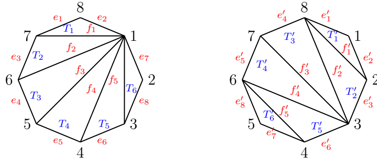
Figure 5: The labelling used to define \phi . Let G_1 be the triangulation graph on the left, and G_2 on the right.
