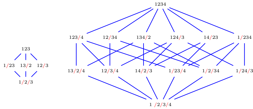
Figure 2: The Kreweras lattices KL(3) and KL(4) .
