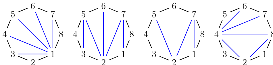
Figure 4: The first and second graphs from the left are triangulation graphs. The third graph is not, because it is not maximal. The graph on the right has an inner triangle, so it is also not a triangulation graph.
