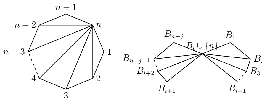
Figure 7: The graph on the left is the spider S_n . The graph on the right is a “double spider.”
