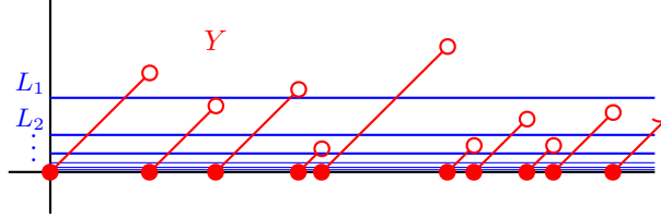
FIGURE 4. A generic sample path of Y and \mathbf{X} , when Y is the age process of a regenerative set as given in Example 2.23.
