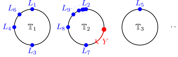
FIGURE 3. As in Example 2.22, we can construct the VMC corresponding to a virtual permutation via Lemma 2.21.
