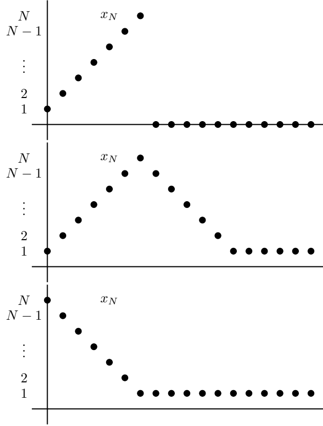
FIGURE 2. The virtual paths of Example 2.10 (top), Example 2.11 (middle), and Example 2.12 (bottom).
