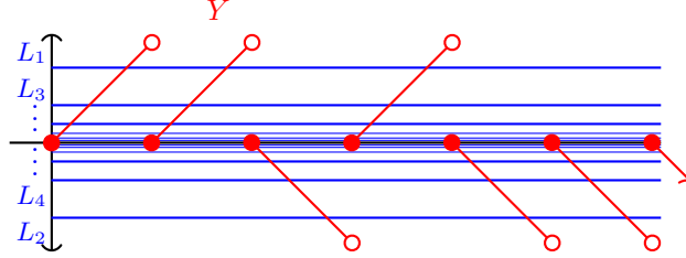
FIGURE 5. A generic sample path of the process Y described by Example 2.24
