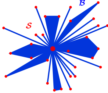
FIGURE 1. A cartoon of the virtual Birkhoff polytope \mathcal{B} (blue) and the virtual permutation matrices \mathcal{S} within it (red).
