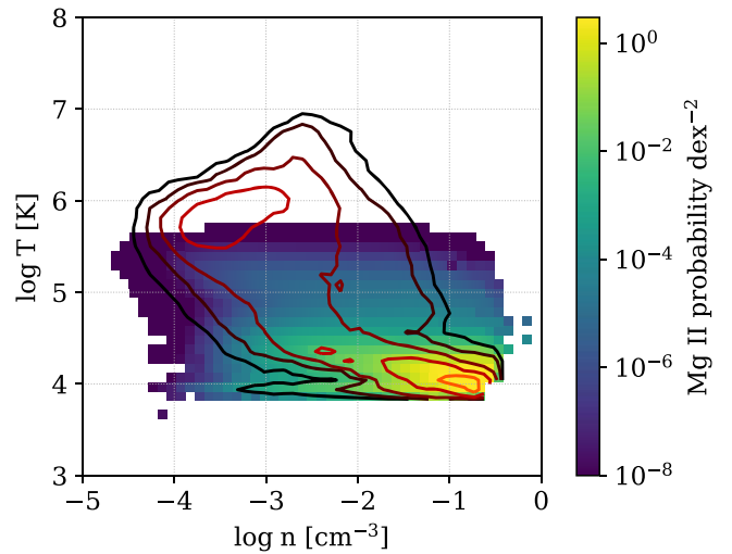
Figure 2. Temperature–number density phase diagram of a single TNG50 halo at z = 1 , colored by the Mg II mass probability density per \text{dex}^2 . Contours show the distribution of all gas mass in the halo.
