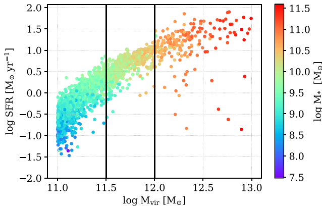
Figure 1. Star formation rate of the central galaxy vs. halo mass for all TNG50 halos between 10^{11} M_{\odot} and 10^{13} M_{\odot} at z = 1 . Each point is colored by the stellar mass of the halo’s central galaxy. Two thick vertical lines demarcate the halo mass range of the fiducial sample.
