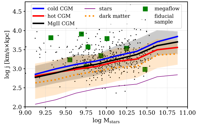
Figure 11. Median-specific angular momentum versus galactic stellar mass for the cold (blue), hot (red), and Mg II (black) CGM as defined in Figure 8, as well as the dark matter halo (dotted orange) and the stellar component of the galaxy (purple) at z = 1 . Unlike previous figures, medians are calculated using a sample of all halos containing central galaxies with stellar masses 10^9 M_{\odot} < M_{*} < 10^{11} M_{\odot} . Shaded regions show the 16th and 84th percentiles of the distributions of the Mg II gas (black), which is similar in size to all components except dark matter (orange), which has noticeably larger scatter. Black points show the Mg II specific angular momentum of the halo-mass-selected fiducial sample that is biased toward higher j for M_{*} \lesssim 10^{9.75} . Green squares show estimations for the specific angular momentum of the major-axis absorbers using inferred rotational velocities from Zabl et al. (2019).
