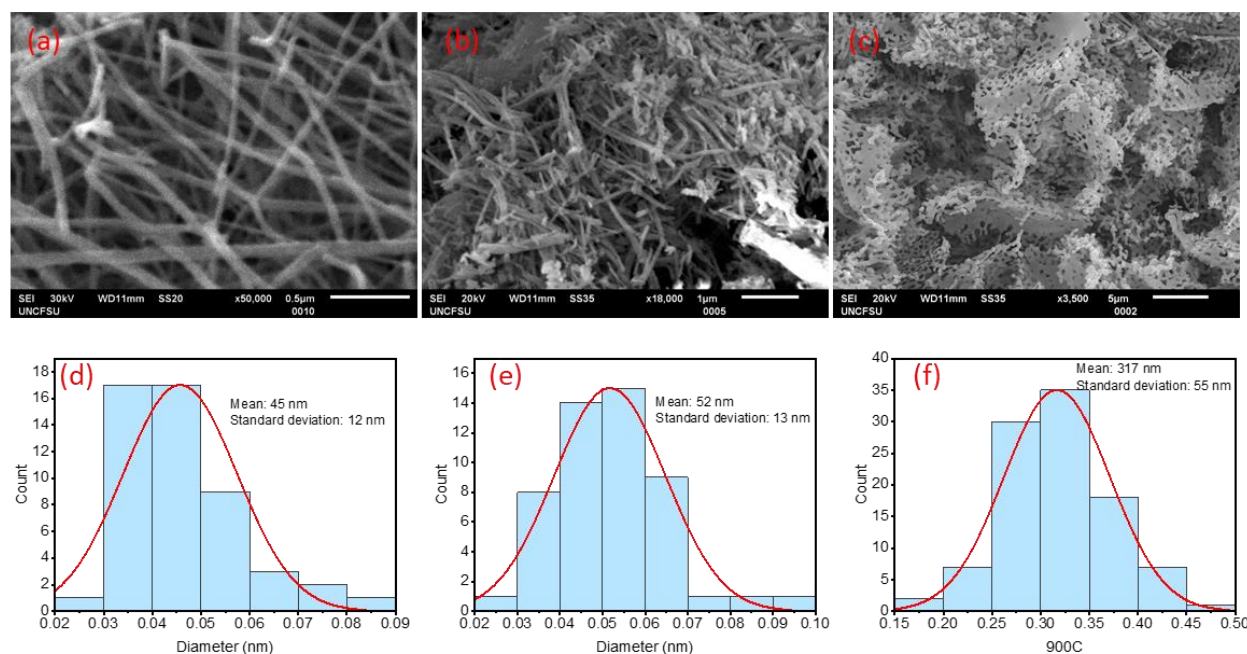
Figure 2. SEM images of samples calcined at 700 °C (a), 800 °C (b), and 900 °C (c), and their diameter distributions (d–f).
