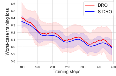
Figure 2: S-DRO significantly reduce loss variances and achieve improved worst-case loss than vanilla DRO.
