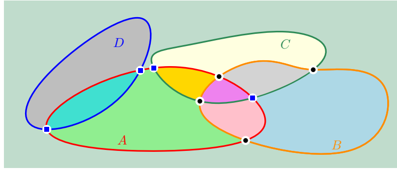
Figure 2: The vertices, elementary arcs, and faces of dimension two formed by the collection \mathcal{S}' = \{A, B, C, D\} of pseudodisks are shown as points (filled squares/circles), arcs, and solid regions, respectively. For \mathcal{R}' = \{A, C, D\} the vertices appearing on \mathcal{U}(\mathcal{R}') are shown as blue squares.
