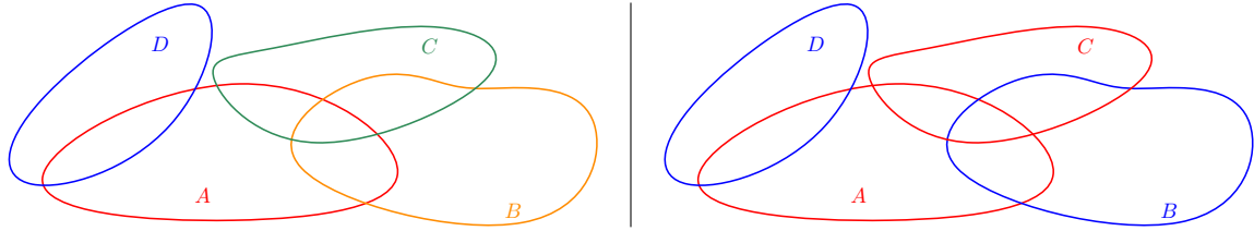
Figure 1: Left: \mathcal{S}' = \{A, B, C, D\} is a set of closed Jordan domains that intersect nicely, and hence is a collection of pseudodisks. Right: \mathcal{S} = \{A \cup C, B \cup D\} is a collection of 2-pseudodisks.
