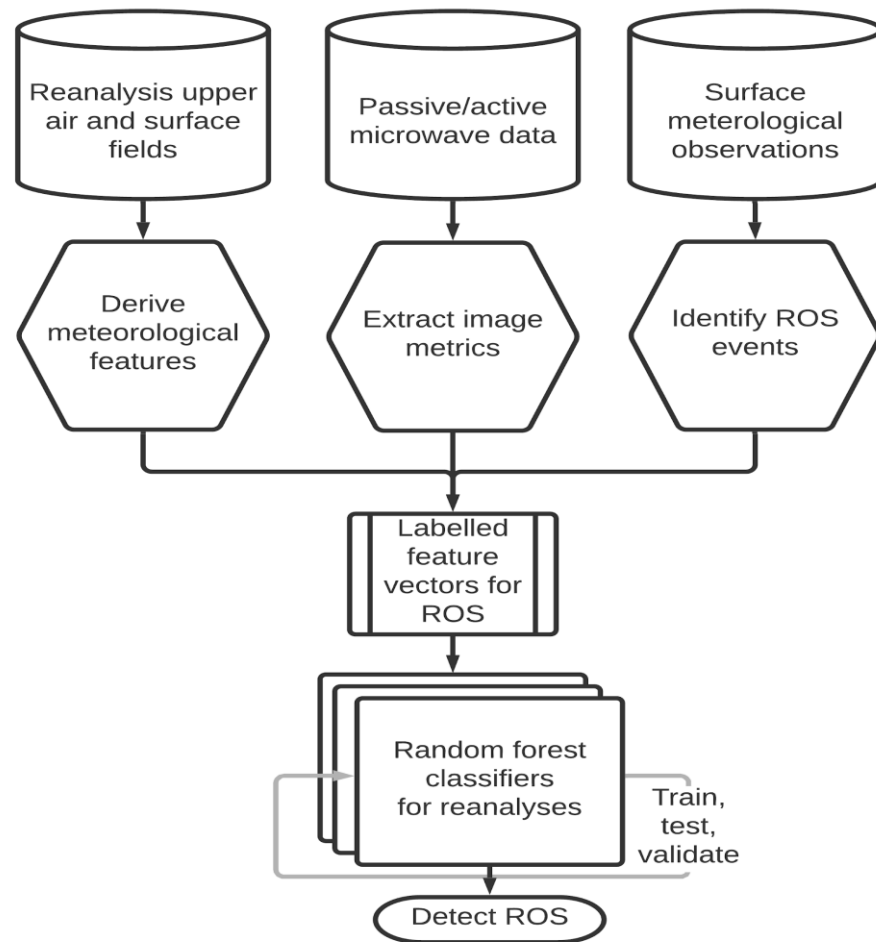
Figure 9. Flow diagram showing potential inputs, and procedure for creating training data and developing the ROS detection algorithm.
