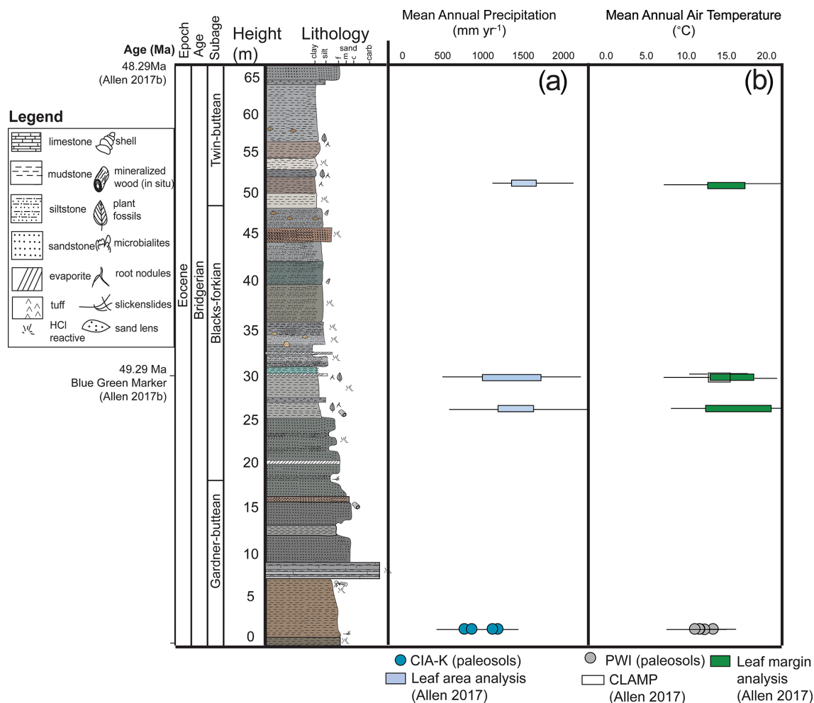
Figure 6. Stratigraphic column with climate proxies. (a) Reconstructed mean annual precipitation (mm yr -1 ) and (b) mean annual air temperature (°C). The boxes are ranges reconstructed for physiognomic proxies, and the circles are values reconstructed using paleosols. The lines for both are established errors for the proxies used based on the initial proxy calibrations. Errors were calculated for each estimate, and the error bars span the total range of calculated error. More information on error can be found within these proxy calibrations (e.g., Wilf, 2000; Sheldon et al., 2002; Spicer et al., 2009; Gallagher and Sheldon, 2013).
