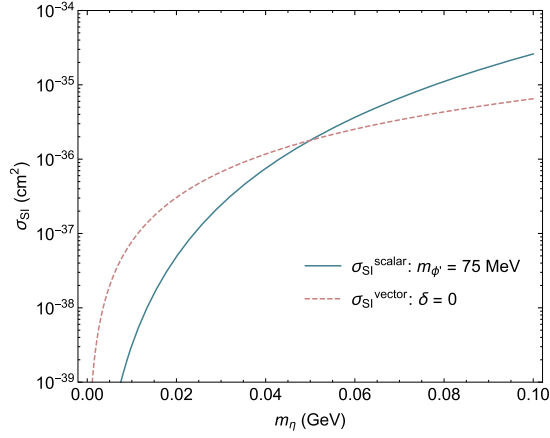
FIG. 4. Spin-independent dark matter-nucleon scattering cross section as a function of the dark matter mass. The blue (solid) line shows the spin-independent (SI) elastic scattering cross section mediated by \phi' for m_{\phi'} = 75 MeV. And the orange (dashed) line shows the SI inelastic scattering cross section mediated by A' with \delta = 0 .
