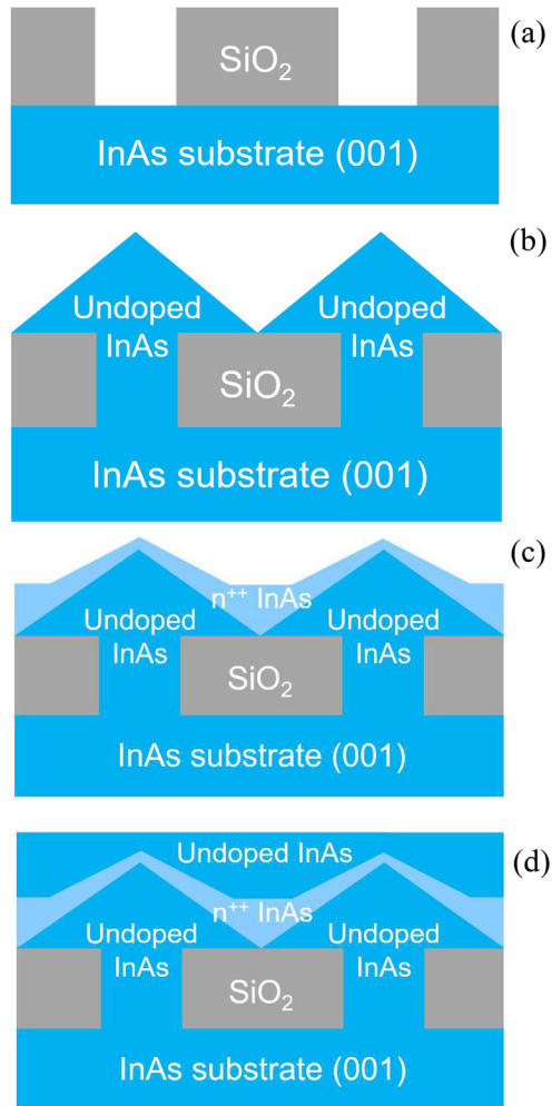
FIG. 2. Cross section illustration of the growth process for embedded plasmonic InAs corrugations. (a) SiO 2 gratings were patterned along the [010] crystal plane direction of a (001) InAs substrate. (b) Lateral overgrowth of undoped InAs was seeded between the gratings using periodic supply epitaxy. (c) Highly n-type doped InAs was then grown on the faceted undoped InAs features. (d) Finally, undoped InAs was grown to return to a planar (001) surface above the plasmonic corrugations.
