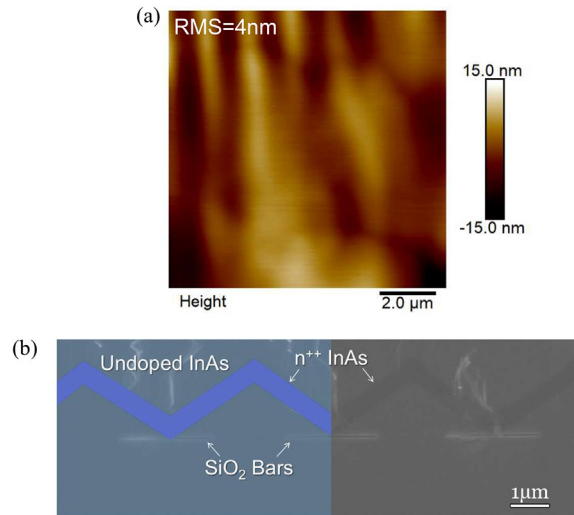
FIG. 4. (a) Atomic force microscope (AFM) image of the planarized plasmonic InAs corrugations showing that the (001) crystal surface has been recovered to a roughness of 4 nm RMS over a 10 \times 10 \mu\text{m}^2 area. (b) Cross-sectional scanning electron microscope (SEM) image of the planarized plasmonic InAs corrugations.
