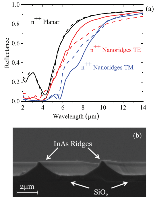
FIG. 3. (a) Fourier transform infrared (FTIR) spectroscopy (solid lines) and Drude model fitting (dashed) TE and TM reflection spectra comparing planar plasmonic InAs and 3.0 μm pitch plasmonic InAs nanoridges. (b) Cross-sectional scanning electron microscope (SEM) images of the InAs corrugations.
