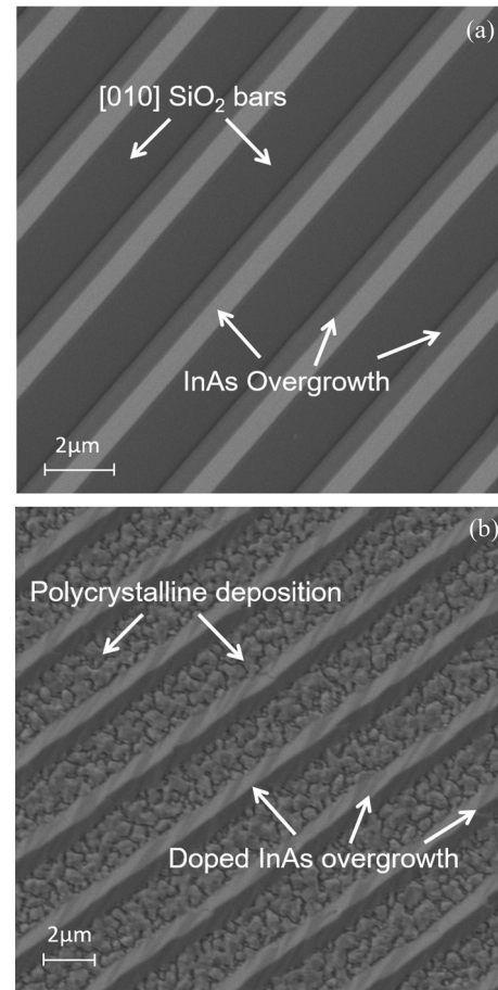
FIG. 1. Plan view scanning electron microscope images of PSE-grown InAs (a) without and (b) with high Si doping.
