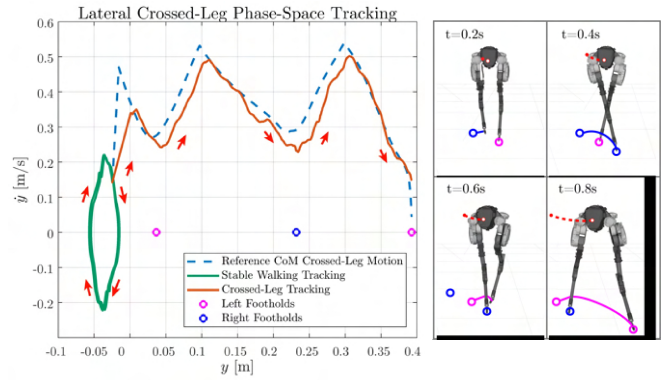
Fig. 8: Cassie is given a 0.4 m/s laterally disturbance from a 0.5 m/s stable forward walking. Cassie successfully executes a leg crossing maneuver.
