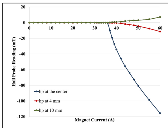
Figure 6: Three Hall probe responses against 250 \mu m thick niobium substrate at 1.97 K. First penetrated flux is detected at 192.5 \pm 2.8 mT.
