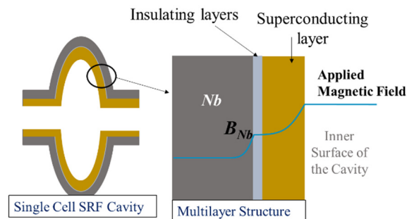
Figure 1: SIS multilayers fabricated on niobium cavity enhances peak surface magnetic field at inner cavity surface.
