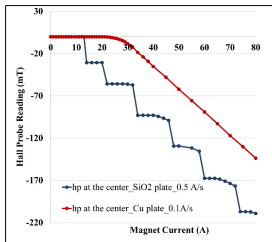
Figure 8: The measurement of Nb 3 Sn/Al 2 O 3 multilayers on Al 2 O 3 wafer grown at University of Wisconsin [20].
