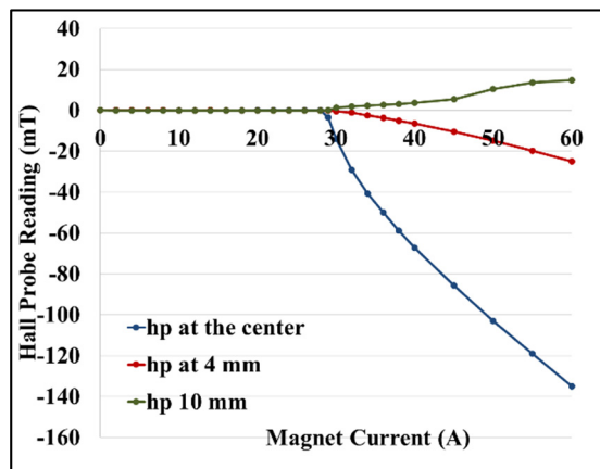
Figure 5: Three Hall probe responses against 250 \mu m thick niobium substrate at 4.35 K. First penetrated flux is detected at 154.0 \pm 2.8 mT.
