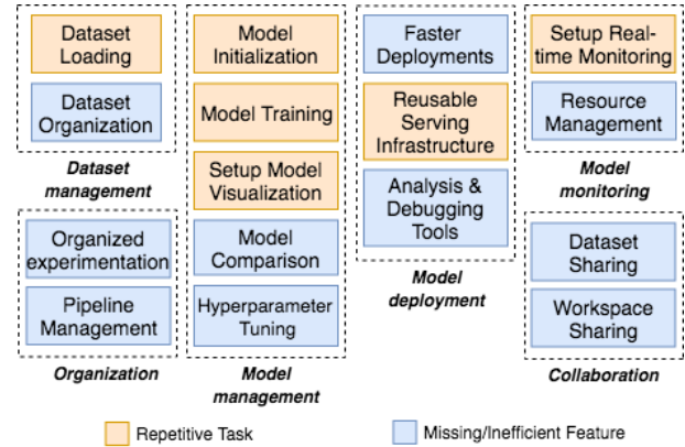
Figure 7: There are a number of repetitive tasks in end-to-end process and some missing features in existing platforms. These can be clustered into reusable components.
