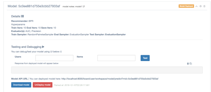
Figure 4: UI (with testing) for a deployed model
