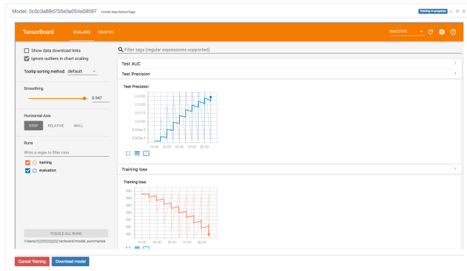
Figure 3: Real-time model variables visualization during training and testing using TensorBoard.
