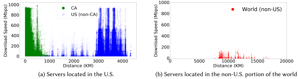
Fig. 2. Download Speed of Measurements for Different Server Locations.
