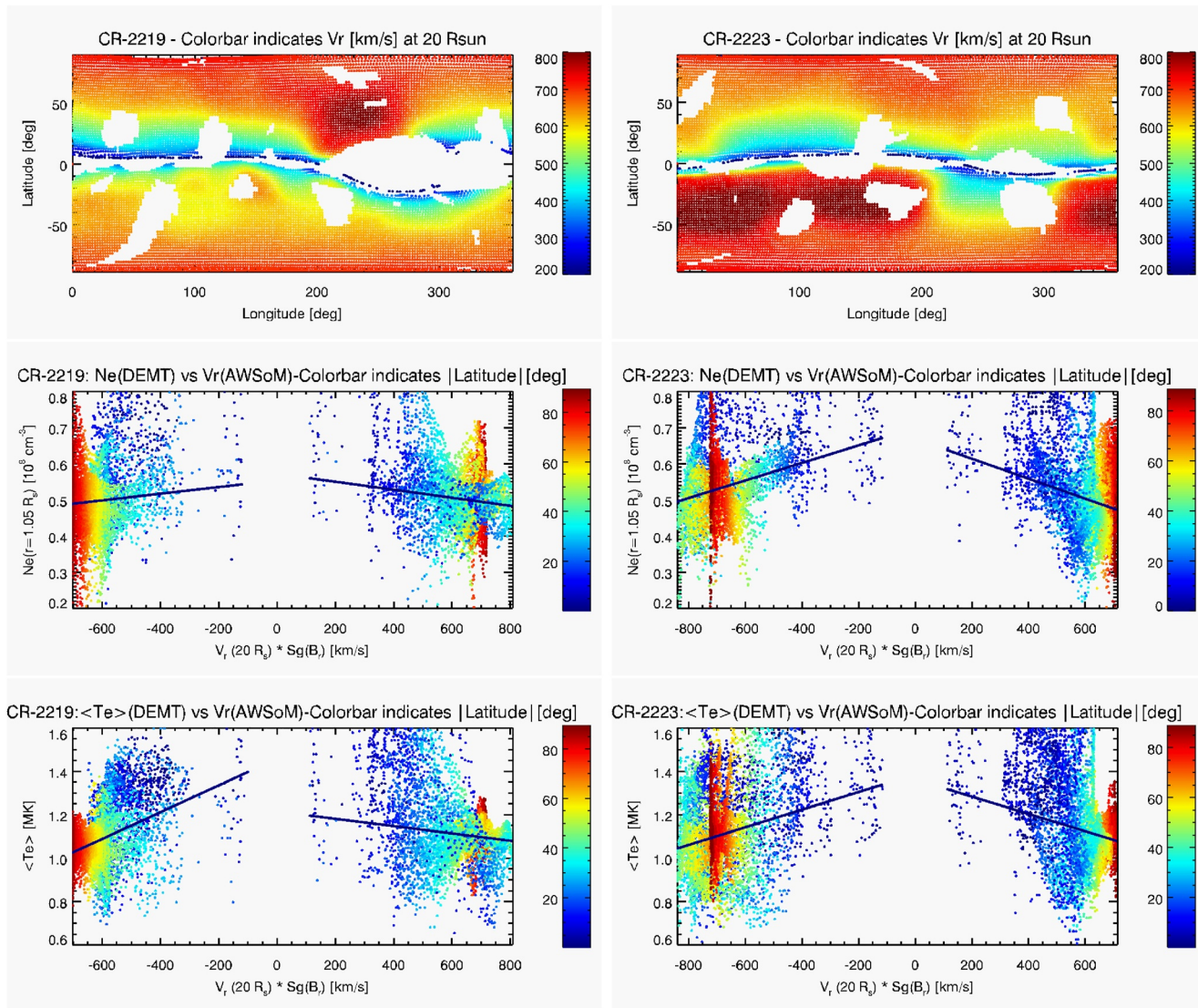
Figure 13. Top panels: latitude-longitude maps of the radial component of the Alfvén Wave Solar atmosphere Model (AWSoM) model terminal solar wind speed V_r(r_M = 20 R_\odot) [km s -1 ], for CR-2219 (left panel) and CR-2223 (right panel), where each dot corresponds to a traced open field line that effectively threads a CH according to the differential emission measure tomography (DEMT) reconstructions (see text in Section 3.3). Middle panels: scatter plots of the DENT coronal base density N_e(r = 1.05 R_\odot) versus the AWSoM model terminal wind speed V_r(r_M) signed by B_r (i.e., multiplied by \text{Sgn}(B_r) ), for all field lines indicated in the top panels. Abscissa negative values correspond to the southern hemisphere and positive ones to the northern hemisphere. Bottom panels: scatter plots of the DENT field line averaged electron temperature \langle T_e \rangle versus \text{Sg}(B_r) V_r(r_M) , for the same field lines. In the middle and bottom panels, straight lines indicate the best Theil-Sen estimator linear fit to the data in each hemisphere. The colorbars indicate the module of the heliocentric latitude of the field line at heliocentric height r_M .
