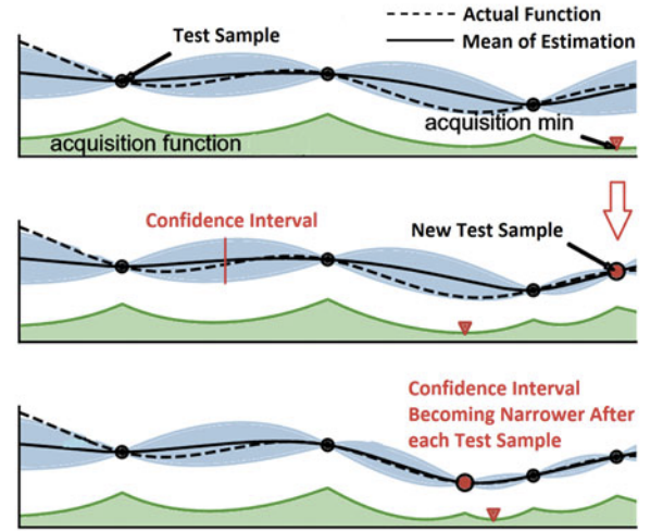
Fig. 2. Illustrative example to show how BO works (adapted with modification from [6]). EI finds the configuration corresponding as global extremum (minimum in this sample) and selects that as the next example.
