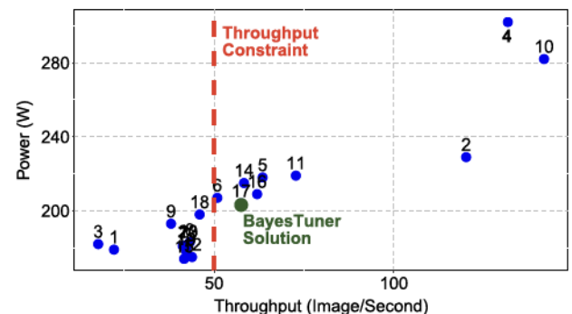
Fig. 6. Detailed behavior of BayesTuner for MobilenetV2 DNN.
