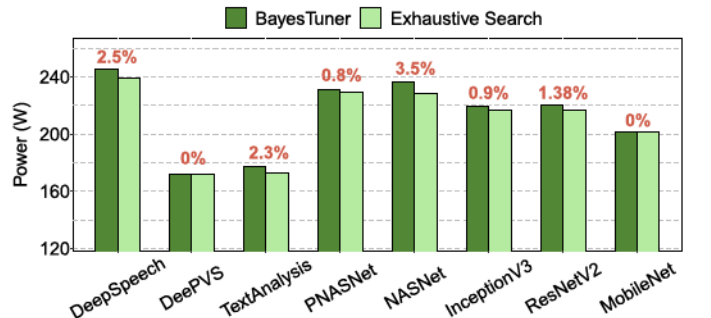
Fig. 4. Comparing the results of BayesTuner against optimal solution for power consumption. The red numbers on top of the bars indicate the difference between BayesTuner and optimal solution. The number of test samples for BayesTuner is 20 and for Exhaustive search is 224.
