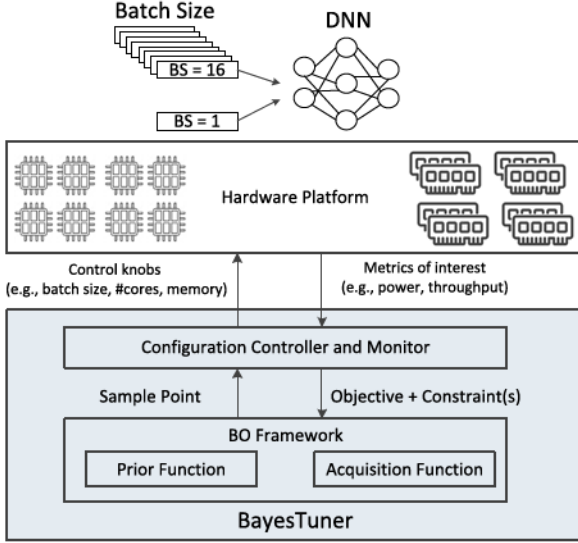
Fig. 3. Overall flow of BayesTuner.
