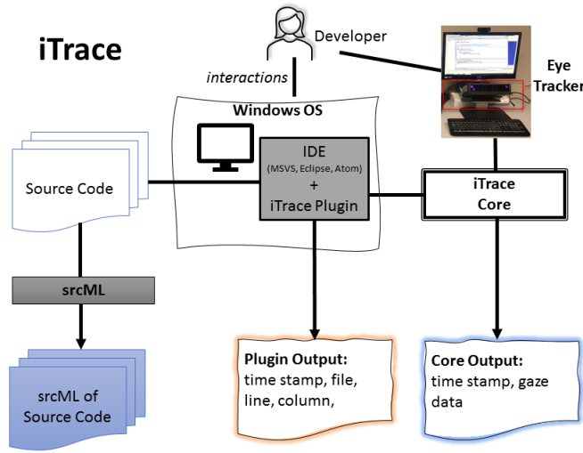
Fig. 2: iTrace Architecture Diagram. iTrace is composed of two main components: the core and an IDE plugin(s). The core interacts with the eye tracker and sends information to the plugin. Given the screen (x, y) coordinate of a gaze, the plugin determines the file, line, and column that maps to that gaze.
