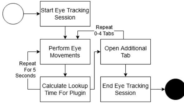
Fig. 9: Process diagram for data collection in Experiment 1 (Data Collection without Deja Vu).
