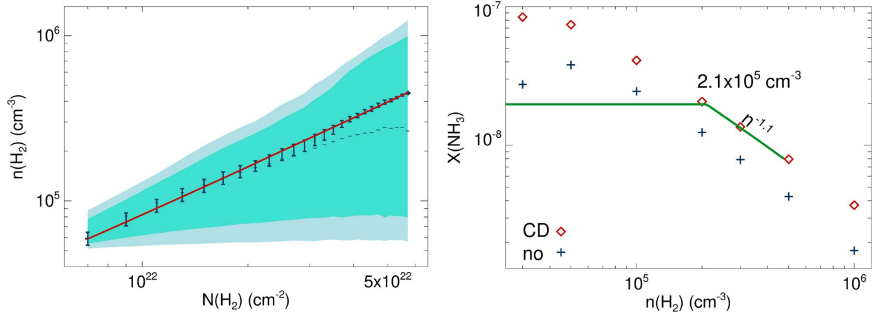
Figure 10. Left: gas density, n(\text{H}_2) , as a function of the \text{H}_2 column density in a 3D model of the H-MM1 core (see text). The shaded regions show the densities between the 5th and 95th percentile (pale blue) and between the 16th and 84th percentile (turquoise) within a certain column density bin. The red line shows a linear fit to the weighted mean densities, \bar{n}(\text{H}_2) , where each LOS is weighted according to standard deviation of the density ( 1/\sigma_n^2 ) along that LOS. The error bars correspond to the weighted sigmas of the sample densities. The median density in each N(\text{H}_2) bin is shown with small horizontal bars. Right: fractional \text{NH}_3 abundance as a function of gas density in H-MM1. The relationship is derived by fitting a broken line to mean \text{NH}_3 column densities below and above the turning point N(\text{H}_2) = 2.6 \times 10^{22} \text{ cm}^{-2} (see Section 3.4), and using a linear fit to \bar{n}(\text{H}_2) vs. N(\text{H}_2) on the left. Also shown are predictions from our chemistry model including chemical desorption (CD; diamonds) and CD turned off (plus signs; see text).
