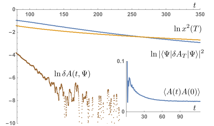
FIG. 2. Plots of the lhs and the rhs of Eq. (11) in logarithmic scale: \ln |\langle \Psi | \delta A_T | \Psi \rangle|^2 (blue lines) and \ln x^2(T) (orange lines). Also shown in brown is \ln \delta A(t, \Psi) . Its approximately linear form (before saturation) confirms exponential decay (3). Inset: plot of the autocorrelation function. All plots are for a nonintegrable Ising spin chain with L = 24 spins with open bc; see Supplemental Material [34] for details.
