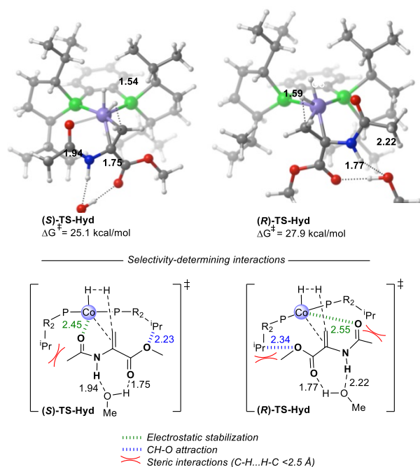
Figure 5. Optimized pro-(S) and pro-(R) transition states for oxidative hydride transfer for (R,R)-( i PuPhos)Co-catalyzed hydrogenation of MAA by redox mechanism A , with a hydrogen-bonded MeOH (barriers relative to 1-MAA, 298K, PBE0-D3BJ,IEFPCM[methanol]).
