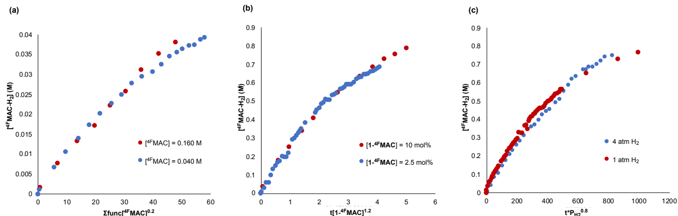
Figure 4. Overlay plots obtained from VTNA for the determination of the rate law for the hydrogenation of 4^{\text{F}} MAC with \text{H}_2 with 1- 4^{\text{F}} MAC as the precatalyst: (a) order in 4^{\text{F}} MAC, (b) order in 1- 4^{\text{F}} MAC , (c) order in \text{H}_2 pressure.
