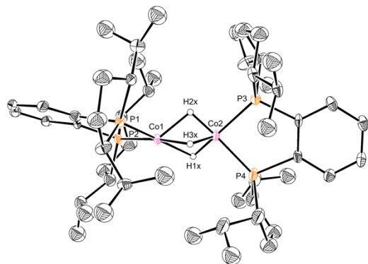
Figure 3. Solid-state structure of [(R,R)\text{-}(\text{iPr-DuPhos})\text{Co}]_2(\mu\text{-H})_3(\text{H}) ( 2 ) at 30% probability ellipsoids with hydrogen atoms, except for the bridging cobalt-hydrides, omitted for clarity.
