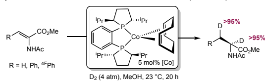
b) Measurement of a KIE for the hydrogenation of 4 FMAC.
