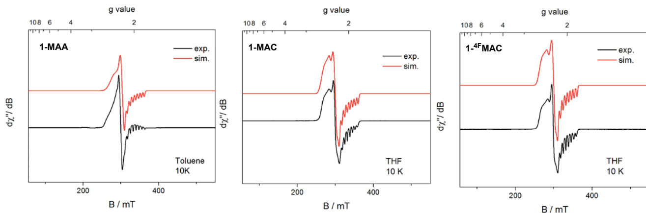
Figure 2. X-band EPR spectra of (R,R) -( i\text{Pr} ) _2\text{DuPhos} )Co(MAA) ( 1-MAA ) (simulation parameters: g_x = 2.00 , g_y = 2.23 , g_z = 2.38 ; g_{\text{strain}} = [0.025, 0.045, 0.21] ; A_{xx} = 215 MHz, A_{yy} = 0 MHz, A_{zz} = 0 MHz; A_{\text{strain}} = [30\ 0\ 0] ), (R,R) -( i\text{Pr} ) _2\text{DuPhos} )Co(MAC) ( 1-MAC ) (simulation parameters: g_x = 2.00 , g_y = 2.23 , g_z = 2.44 ; g_{\text{strain}} = [0.027, 0.078, 0.088] ; A_{xx} = 198 MHz, A_{yy} = 0 MHz, A_{zz} = 103 MHz; A_{\text{strain}} = [0\ 0\ 37] ), and (R,R) -( i\text{Pr} ) _2\text{DuPhos} )Co( ^4\text{F} MAC) ( 1- ^4\text{F} MAC ) (simulation parameters: g_x = 2.00 , g_y = 2.22 , g_z = 2.45 ; g_{\text{strain}} = [0.025, 0.072, 0.087] ; A_{xx} = 200 MHz, A_{yy} = 0 MHz, A_{zz} = 102 MHz; A_{\text{strain}} = [0\ 0\ 25] ) at 10 K. Microwave frequency = 9.38 GHz, power = 0.02 mW, and modulation amplitude = 0.4 mT/100 kHz.
