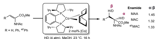
c) Catalytic hydrogenations using hydrogen deuteride (ratios are of deuterium incorporation).
