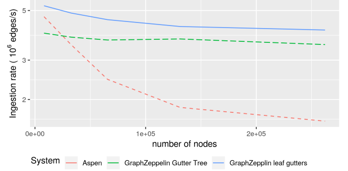
Figure 13: GRAPHZEPPELIN is faster than Aspen and Terrace even when all data structures fit in RAM.
