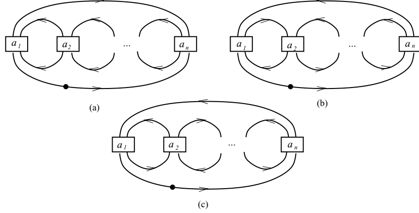
FIGURE 4. Orientation on P . The three diagrams indicate the three combinatorially different orientations: in (a) we show the case when all a_i are odd (hence n is odd), in (b) the case when a_1 is even and n is odd, and finally in (c) the case when a_1 is even and n is even. (The difference between the two last cases is the orientation at the first strand.)
