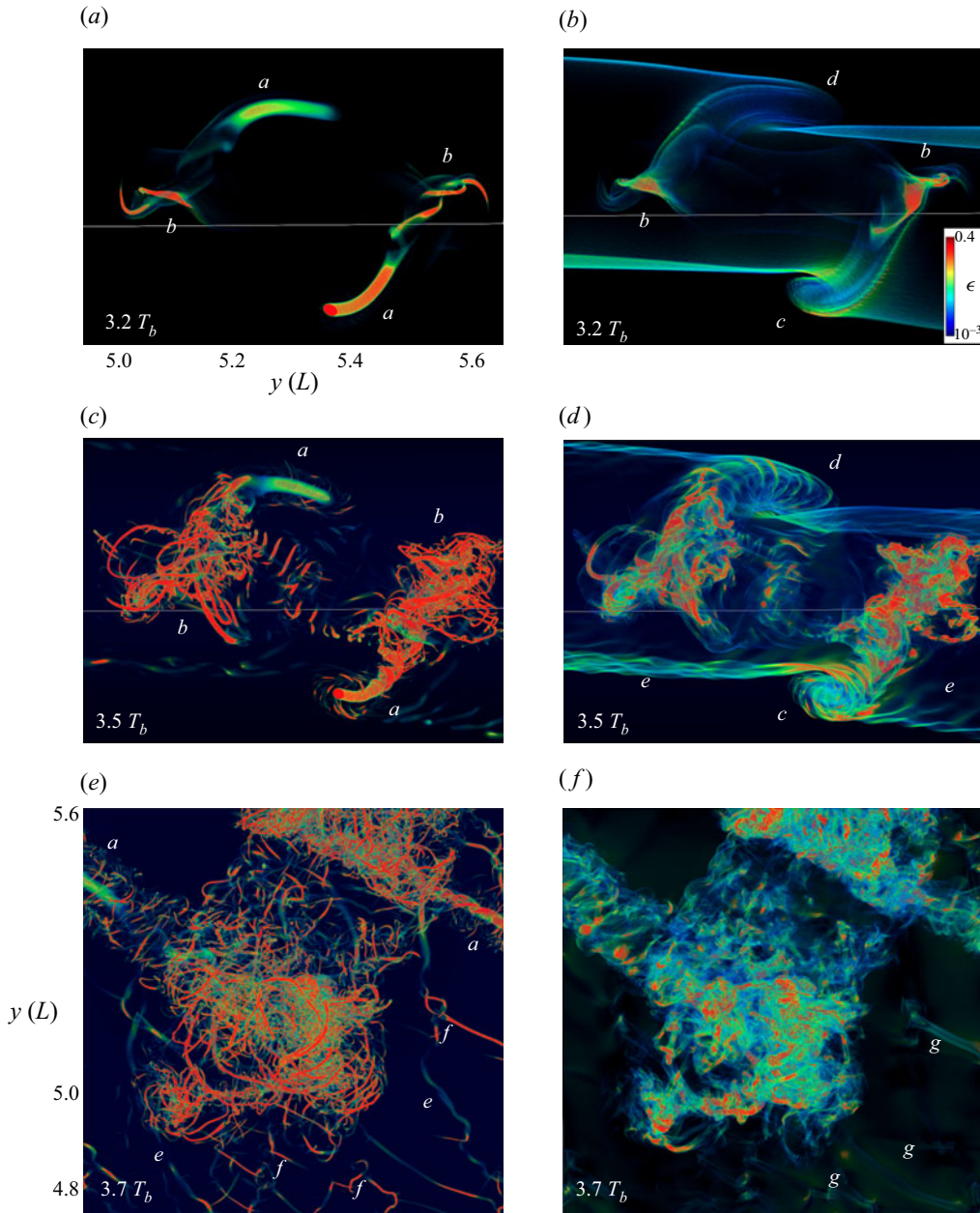
Figure 8. Relations between \lambda_2 and \epsilon (left and right) in region 2 in figure 2 as the vortex dynamics drive turbulence transitions. Views are from larger x and z at 3.2 T_b and from above at 3.5 T_b . Sites labelled a – g are cited in the text. The \epsilon colour scale is logarithmic.
