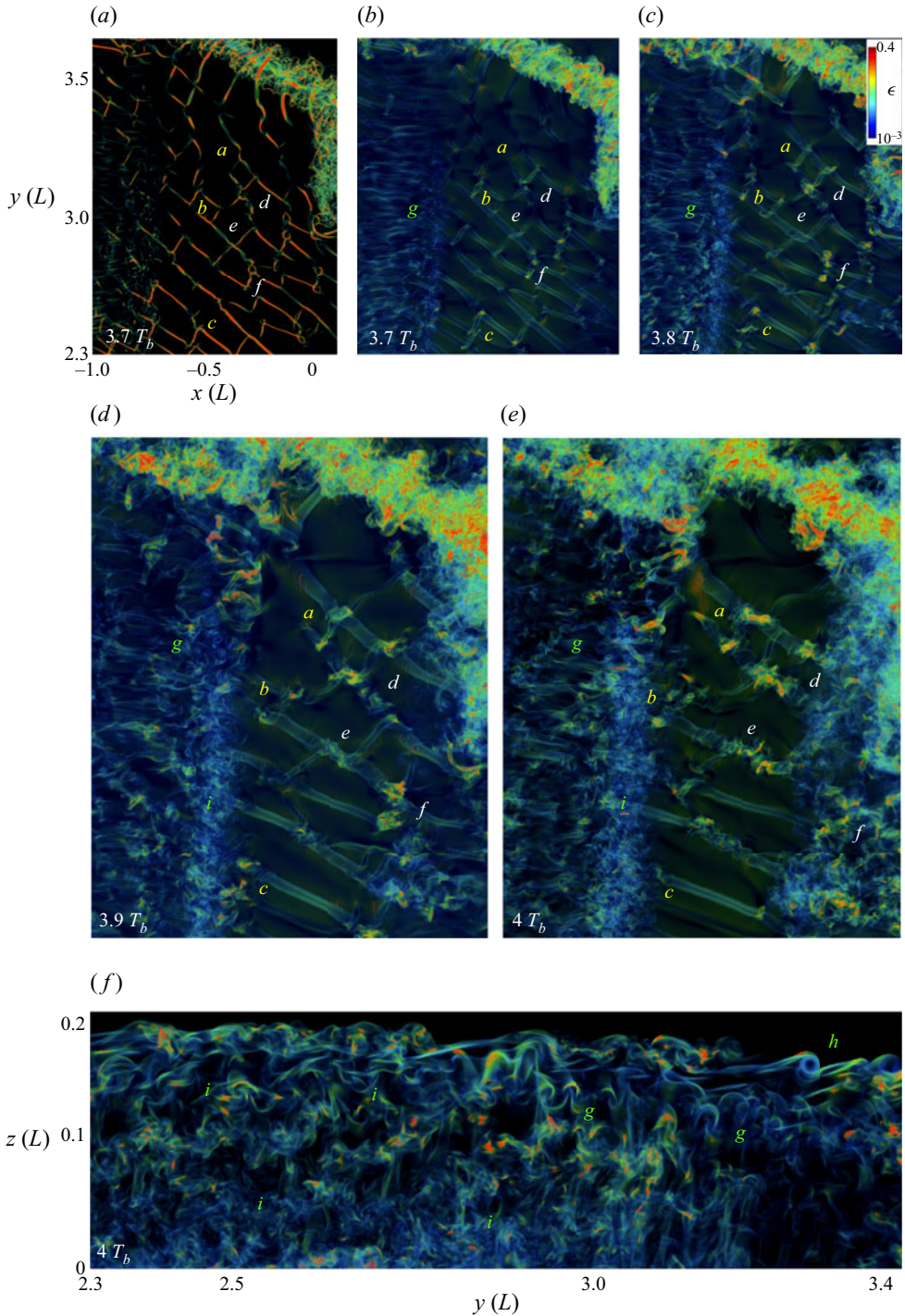
Figure 14. Expanded views of \epsilon imaging in figure 10 at lower left accompanying secondary KHI and CI influenced by type 1 tube and knot dynamics from 3.7\text{--}4T_b . Here, \lambda_2 at 3.7T_b is shown for comparison at upper left with axes appropriate for panels a\text{--}e . An expanded horizontal view of \epsilon for these same dynamics at upper left in figure 11 viewing the forward edge of the rearward KH billow (along x ) at 4T_b with (y, z) axes. Colour scales are as above. Site labels are referred to in the text.
