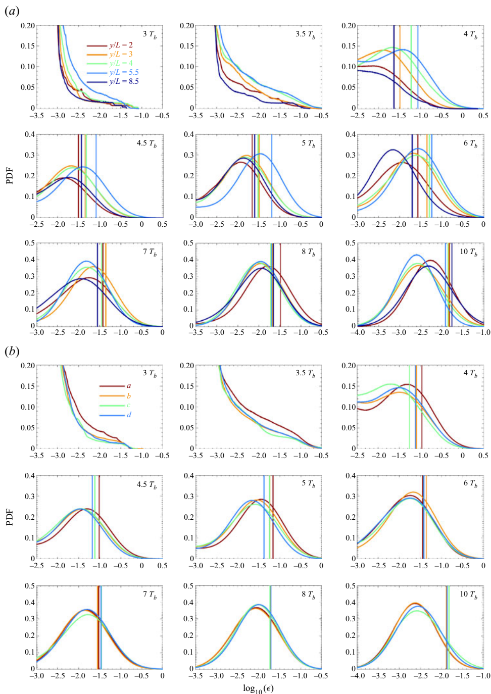
Figure 17. The \epsilon PDFs at y/L = 2, 3, 4, 5.5 and 8.5 for |z| \leq 0.2 and \Delta y/L \leq 0.1 from 3 – 10T_b (a) and for regions a, b, c and d (b) shown in figure 16. Line codes are shown at 3T_b ; vertical lines show \bar{\epsilon} . Note the varying \epsilon scales with time.
