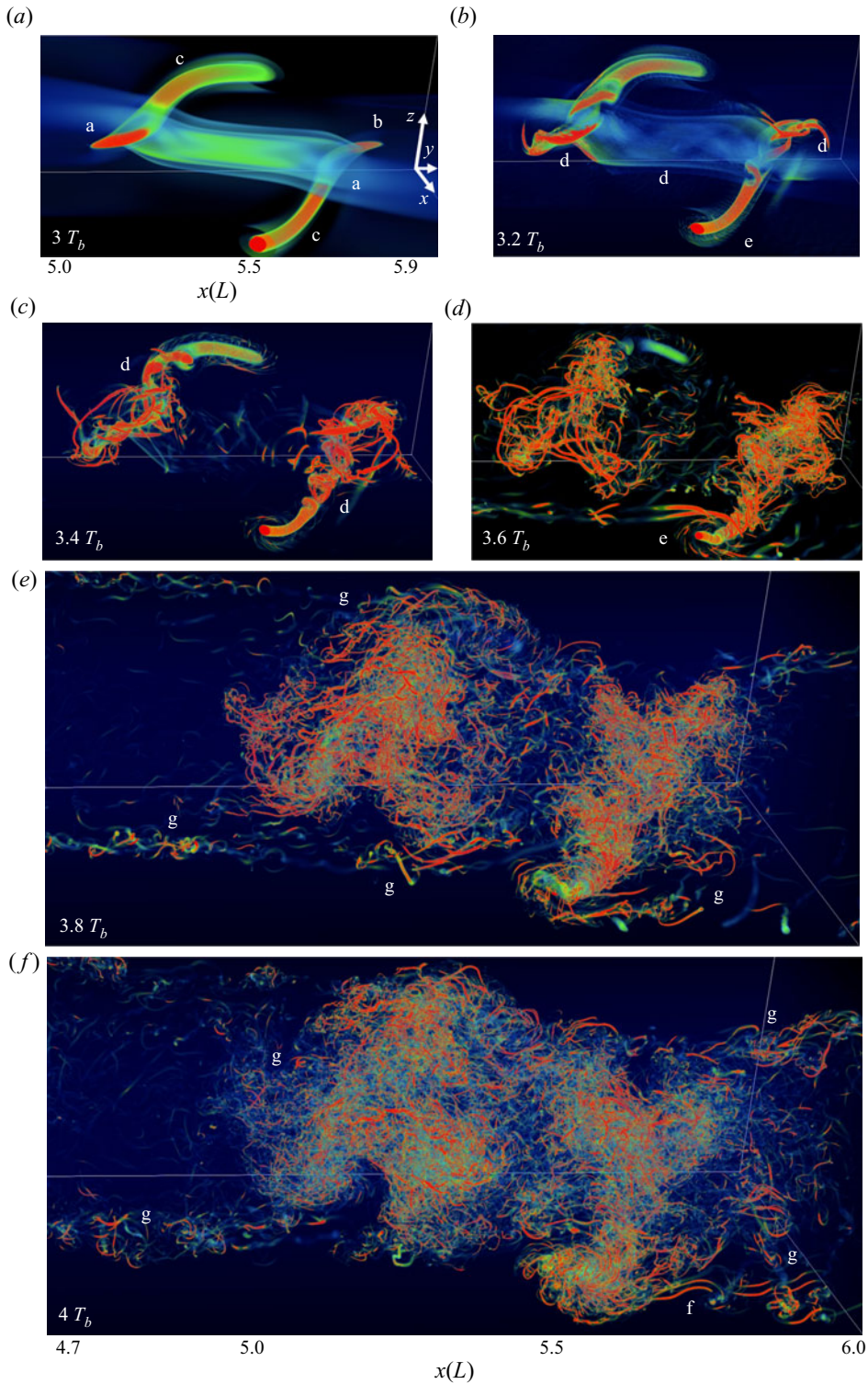
Figure 15. As in figure 13 for \lambda_2 in Region 3 in figure 10 from 3\text{--}4T_b viewed from larger x , smaller y and larger z , and spanning the interval of strong initial KH billow and tube interactions and initial knot dynamics. Earlier times are shown in the upper portion of the full subdomain.
