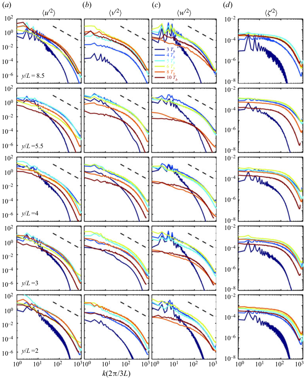
Figure 18. Component variance (panels a–c ) and enstrophy spectra (panel d ) from 3\text{--}10T_b at y/L = 2, 3, 4, 5.5 and 8.5 (bottom to top). Dashed lines show a -5/3 slope.
