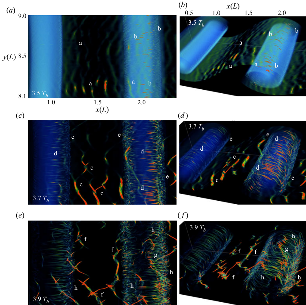
Figure 17. As in figure 12 for \lambda_2 from x/L = 0.5 – 2.5 and y/L = 8 – 9 ( a, c, e ) showing emergence of initial secondary instabilities yielding initial transitions to turbulence. The same 3-D fields are shown at right viewed from larger x , smaller y , and positive z ( b, d, f ). See text for details.
