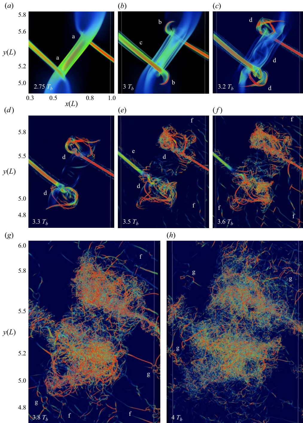
Figure 14. As in figure 12 for \lambda_2 in Region 3 highlighted by the white rectangle in figure 10 viewed from above and spanning times from 2.75–4 T_b (see axes at 2.75 T_b ). Note the more rapid excitation of larger-scale twist waves that drive faster breakdown of the billow core and vortex tubes relative to those seen in Region 2 in figures 12 and 13.
