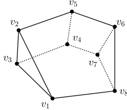
FIGURE 7. An example of a polytope on 8 vertices conjectured to be the maximizer of the number of monotone paths among simple polytopes. f(v_1) < f(v_2) < \dots < f(v_8) .
