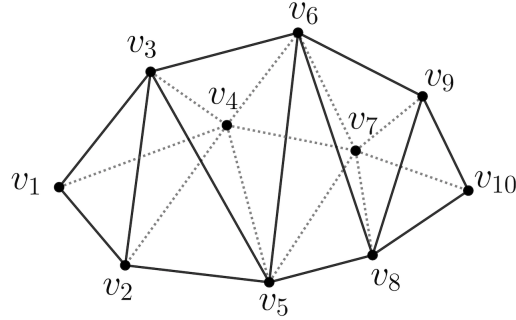
FIGURE 3. Example of the polytope X(10)
