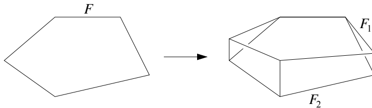
FIGURE 5. The wedge of a pentagon over an edge
