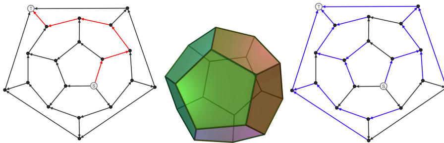
FIGURE 1. The regular dodecahedron (center), with examples of an f -monotone path (left) and an f -arborescence (right) for one of its LP-admissible orientations.
