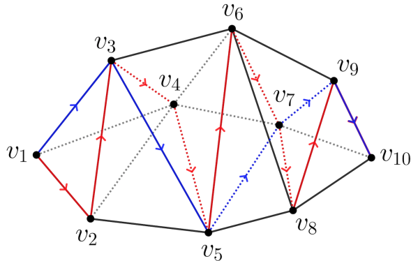
FIGURE 4. Two monotone paths on X(10)
