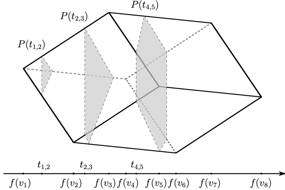
FIGURE 6. A combinatorial cube and some of its fibers
