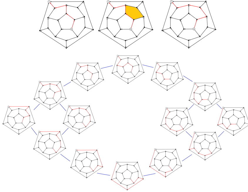
FIGURE 2. A polygon flip on the oriented dodecahedron and the resulting flip graph
