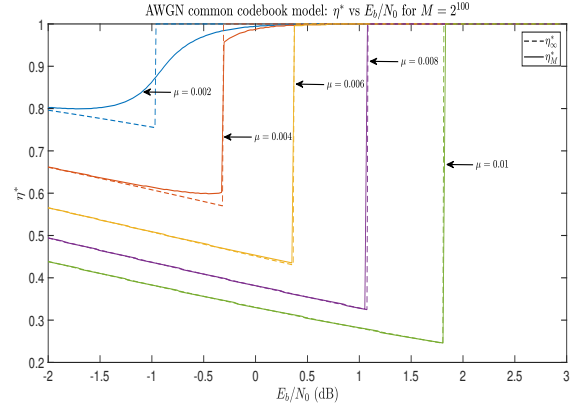
Fig. 5: AWGN same codebook model: \eta^* vs E_b/N_0 for M = 2^{100} . The solid lines correspond to \eta^* \equiv \eta_M^* from (167). The dashed lines correspond to \eta_\infty^* defined in (172).
