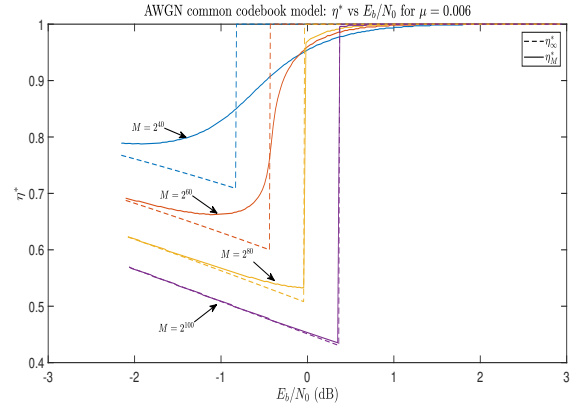
Fig. 6: AWGN same codebook model: \eta^* vs E_b/N_0 for \mu = 0.006 . The solid lines correspond to \eta^* \equiv \eta_M^* from (167). The dashed lines correspond to \eta_\infty^* defined in (172).
