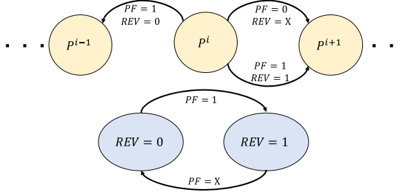
Fig. 13. State transition diagram for Mealy machine-based FSM-1 and FSM-2.
