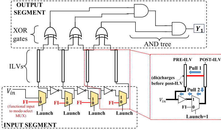
Fig. 1. Simplest form of the BIST architecture and illustration of the hard-short behavior.
