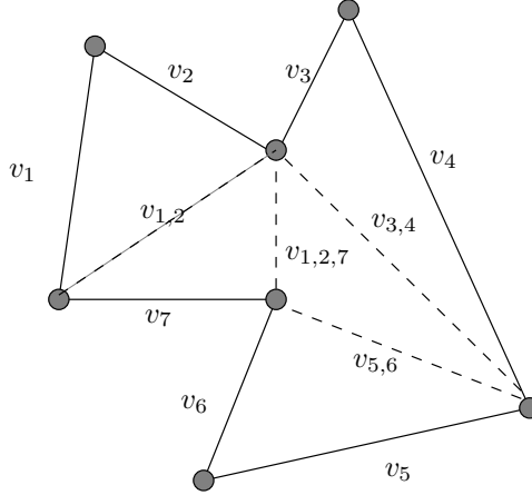
FIGURE 3.2. Triangulated polygon
