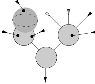
FIGURE 4.4. A treed disk with three disk components and one sphere component
