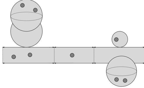
FIGURE 6.1. A stable marked strip
