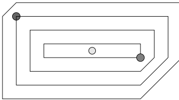
FIGURE 2.2. Moment images of regular tori for the twice blow-up of \mathbb{P}^1 \times \mathbb{P}^1
