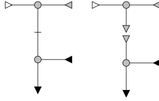
FIGURE 4.6. Cutting an edge
