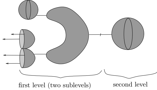
FIGURE 7.2. Broken disk with a boundary node
