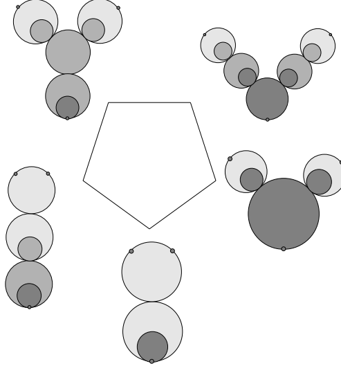
FIGURE 5.6. Twice-quilted disks
