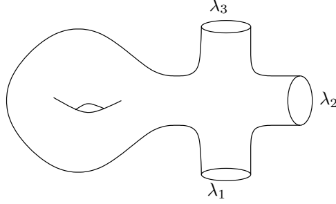
FIGURE 2.3. Compact surface with labelled boundary
