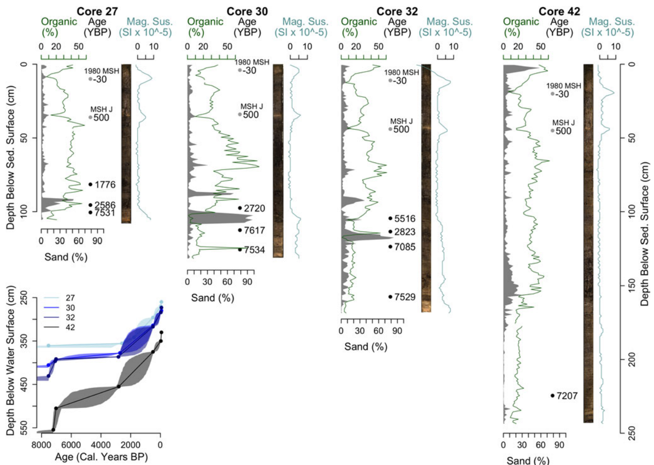
Figure 4. Stratigraphic, sedimentological, chemical, and age data for cores 27, 30, 32, and 42 from Silver Lake include evidence of a low-water phase recorded by high sand content (% inorganic >63\mu\text{m} shaded in gray), low loss-on-ignition at 550^\circ\text{C} (as a measure of sediment organic content, green lines), and changes in magnetic susceptibility (blue lines). Digital photo images show the visual stratigraphy and the age-depth relationships in the cores, including mid-Holocene phases of limited accumulation consistent with shallow water based on calibrated radiocarbon ages (black circles) and tephra ages (gray circles) that are also plotted on bottom left graph, where the shading represents the 95% confidence intervals. MSH is Mount St. Helens.
