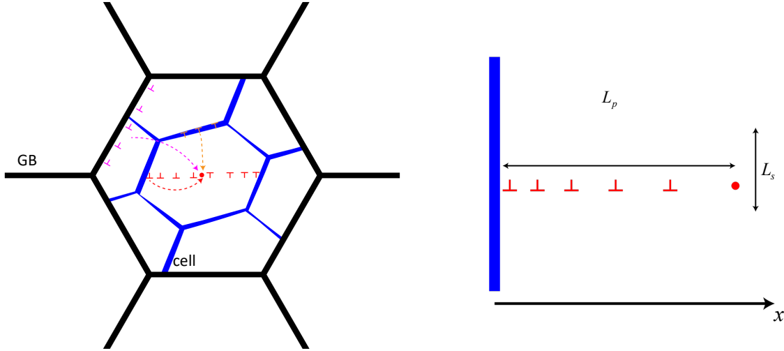
Fig. 4 Schematic illustrations of multiple sources of back stresses. (a) Three sources of back stresses (indicated by colored arrows) acting on a typical dislocation source such as a Frank-Read (FR) source inside a grain (enclosed by grain boundaries (GBs) represented by black segments) containing as-printed dislocation cells enclosed by cell walls (blue segments). (b) A dislocation pile-up against a dislocation cell wall (thick blue line). The distance between the cell wall and the FR source (red dot) is L_p , and the spacing between neighboring pile-ups on parallel slip planes is L_s .
