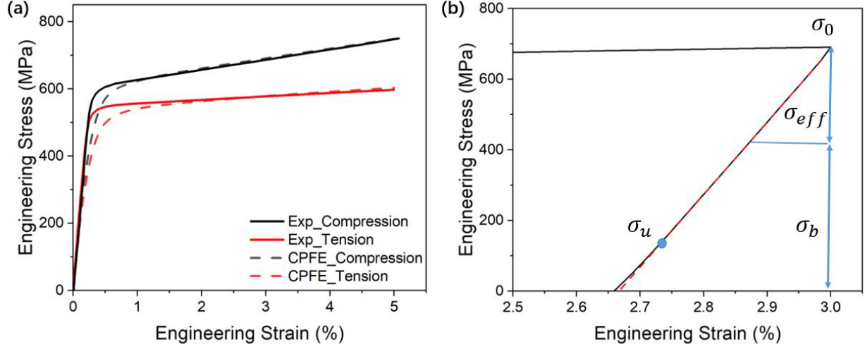
Fig. 7 CPFE simulation results. (a) Comparison of stress-strain curves under uniaxial tension and compression between experiments [9] (solid lines) and CPFE simulations (dashed lines) for as-printed samples. (b) Determination of simulated back stress from an unloading branch using Dickson's method.
