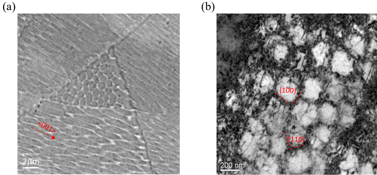
Fig. 1 Coincident chemical cells and dislocation cells in as-printed 316L stainless steel processed using LPBF. (a) SEM image of domains of chemical cells elongated with different orientations. The red arrow indicates that the local cells elongate along the in-plane \langle 001 \rangle direction. (b) TEM image of dislocation cells. The red dashed lines indicate that the cell walls are close to \{100\} and \{110\} .
