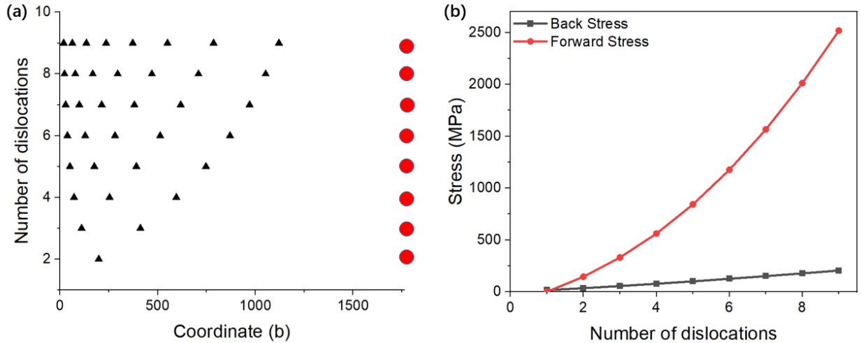
Fig. 5 Numerical results of the dislocation pile-up model in Fig. 4(b). (a) Equilibrium dislocation positions x_j (black triangles) for a dislocation pile-up under different applied resolved shear
