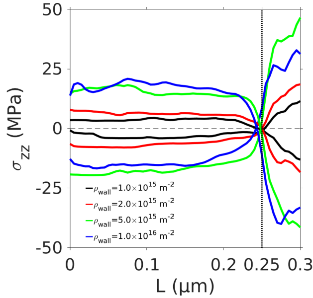
Fig. 3 3D DDD simulation results with different initial dislocation densities in cell walls \rho_{\text{wall}} .
