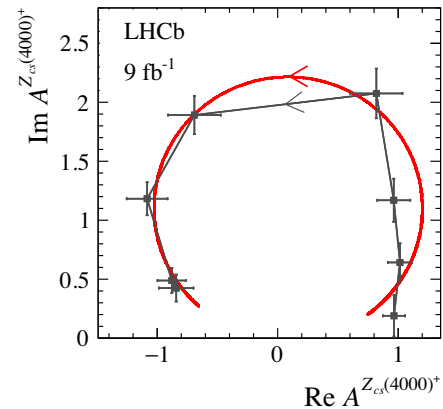
FIG. 5. Fitted values of the Z_{cs}(4000)^+ amplitude in eight m_{J/\psi K^+} intervals, shown on an Argand diagram (black points). The red curve represents the expected Breit-Wigner behavior between -1.4\Gamma_0 and 1.4\Gamma_0 around the Z_{cs}(4000)^+ mass.
