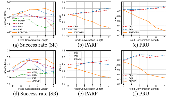
Figure 4: Recommendation performance and popularity bias metrics under different fixed lengths of conversations.
