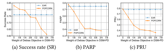
Figure 5: Recommendation performance (SR) and popularity bias (PARP, PRU) results on Movie dataset when varying the weight of the debiasing objective in DSM-PD.
