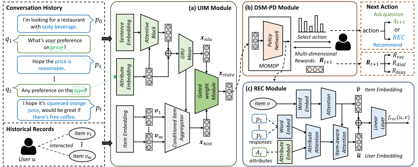
Figure 3: Workflow of our proposed Conversational Recommender System with HitL Popularity Debiasing.
