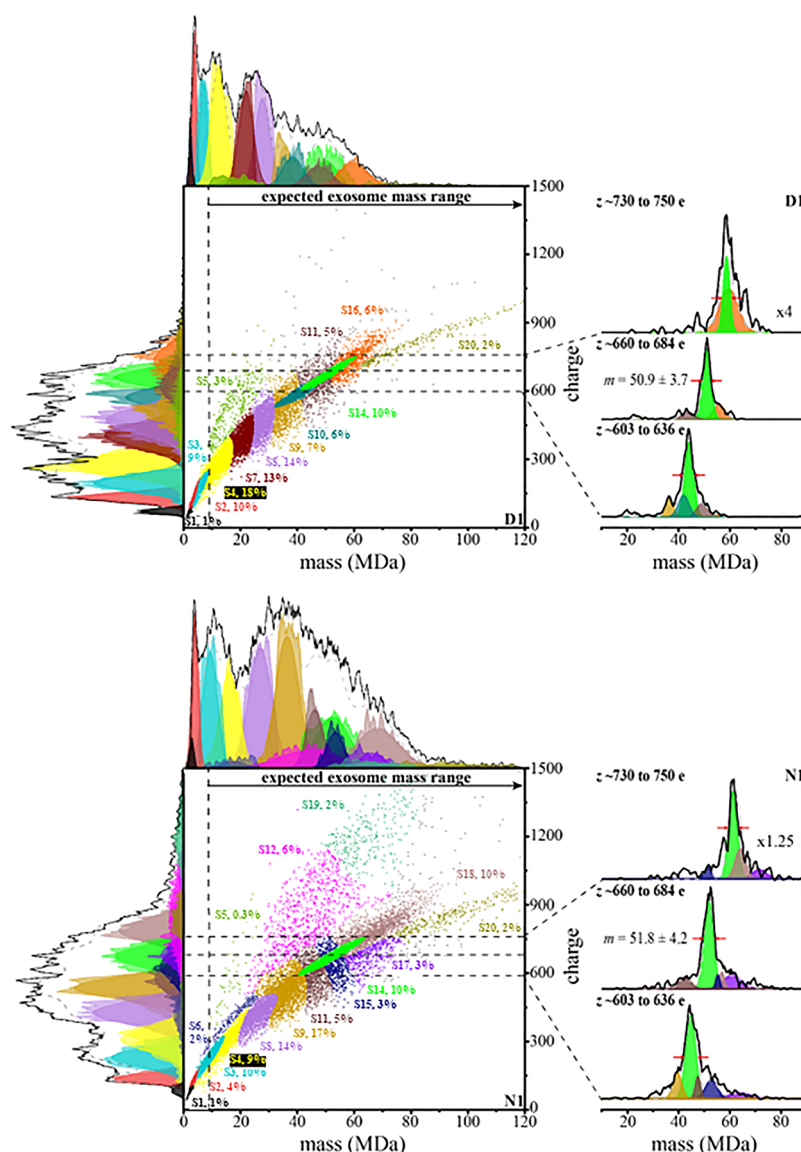
Figure 3. Two-dimensional mass versus charge plot showing subpopulations obtained from Gaussian fits to the experimental data for the first CDMS measurement of nondiabetic and diabetic \text{Exo}_k samples. See the text for details. This model finds evidence for 15 and 13 subpopulations with abundances over 1% for nondiabetic and diabetic samples, respectively. Each point represents the mass and charge measured for a single particle and is assigned to a subpopulation (indicated by a color). Subfamily assignment is based on the highest probability of each particle belonging to a specific subfamily. Visually, this assignment leads to boundaries that are artificially strict when in reality the subpopulations overlap. The top and left side traces show the integrated raw data for the mass and charge dimensions, respectively, and the corresponding sums of the Gaussian curves as black lines for these dimensions. The determined fits for each subpopulation are also shown and delineated using the same color scheme. The percentage of each subpopulation is also indicated. The dashed vertical line provides an estimate of the delineation between those particles having masses in the range that is expected for exosomes and those particles that are too small to be exosomes. To the right of both the N1 and D1 mass versus charge plots is the integrated mass distribution of the N1 and D1 \text{Exo}_k at specified charge ranges (described above, horizontal dashed lines visually show these regions) corresponding to cross sections of the densely populated S14 subpopulation. The S9, S10, S11, S15, S16, S17, and S18 subpopulation mass distributions are also included. The data were normalized to 1 and treated as a composite data set. Mass spectra generated upon integrating the ion signal across the charge dimension used 0.45 MDa bins.
