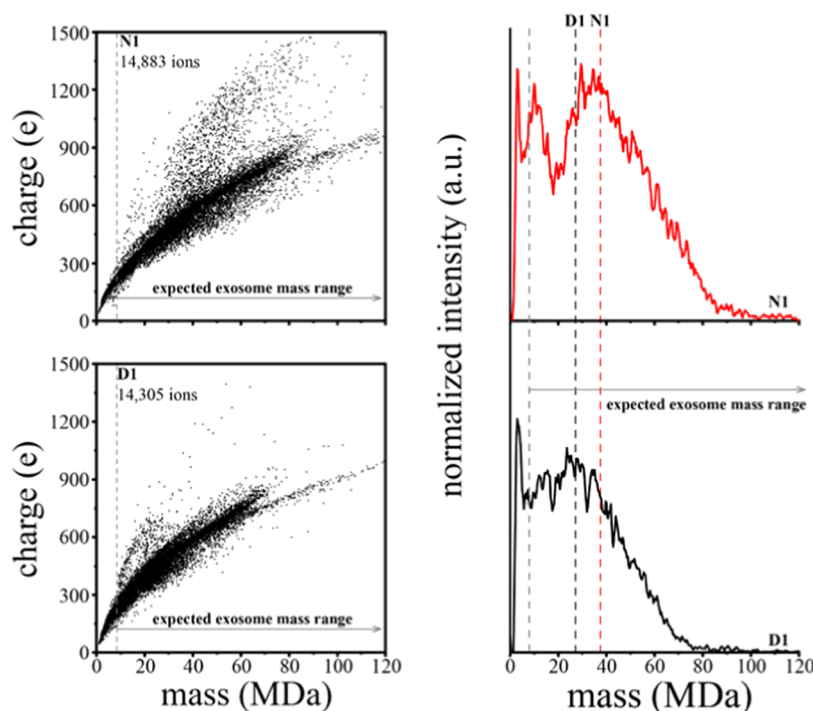
Figure 1. (a, b) Mass versus charge CDMS measurements for nondiabetic (N1) and diabetic (D1) wound-edge keratinocyte-derived exosome samples. (c) N1 (red trace) and D1 (black trace) mass spectra generated upon integrating the ion signal across the charge dimension using 0.35 MDa bins. Red (N1) and black (D1) dashed lines mark the average mass. The gray line denotes the expected mass range of exosomes based on assuming a spherical geometry, a 30 nm minimum exosome diameter, and an average density of 1.17 g/mL.
