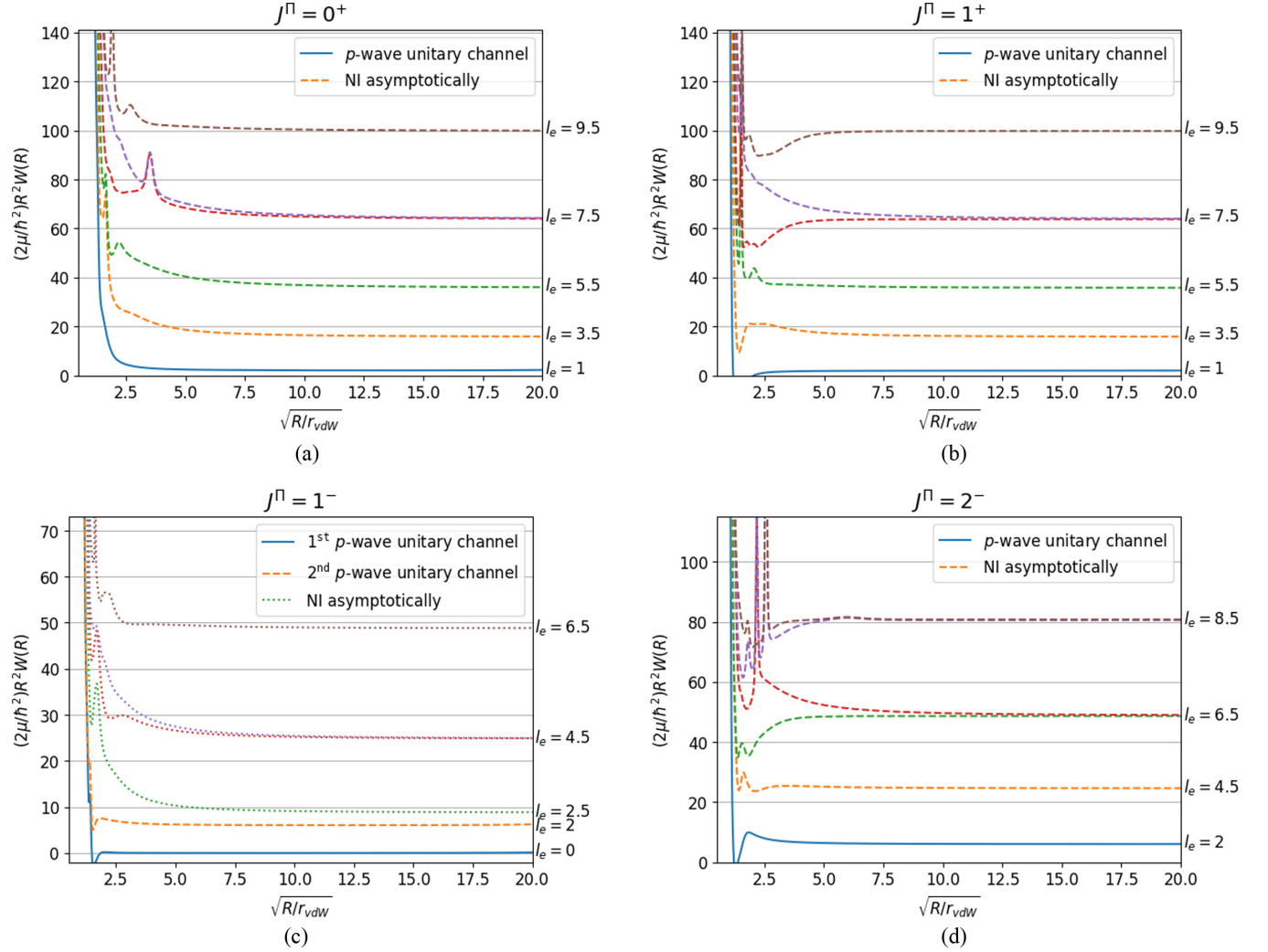
FIG. 3. The adiabatic potential curves for the first to sixth channels vs hyperradius for the two-component three-fermion system ( \downarrow\uparrow\uparrow ), with the interaction between fermions in different spin states set at the p -wave unitary limit ( V_p \rightarrow \infty ) and the interaction between the same spin state fermions set at a weak value with p -wave scattering volume close to V_p = -2 r_{\text{vdW}}^3 for several symmetries J^\Pi . (a), (b) The solid (blue) curve corresponds to the p -wave unitary channel, and the coefficient of 1/(2\mu R^2) is approximately 2. (c) The solid (blue) curve and dashed (orange) curve exhibit the p -wave universal property, and their asymptotic coefficients of 1/(2\mu R^2) are computed to have the values \approx 0 and \approx 6 , respectively. (d) The lowest adiabatic potential curve (solid curve) represents the p -wave unitary channel, and the asymptotic 1/(2\mu R^2) coefficient is calculated to have the value \approx 6 .
