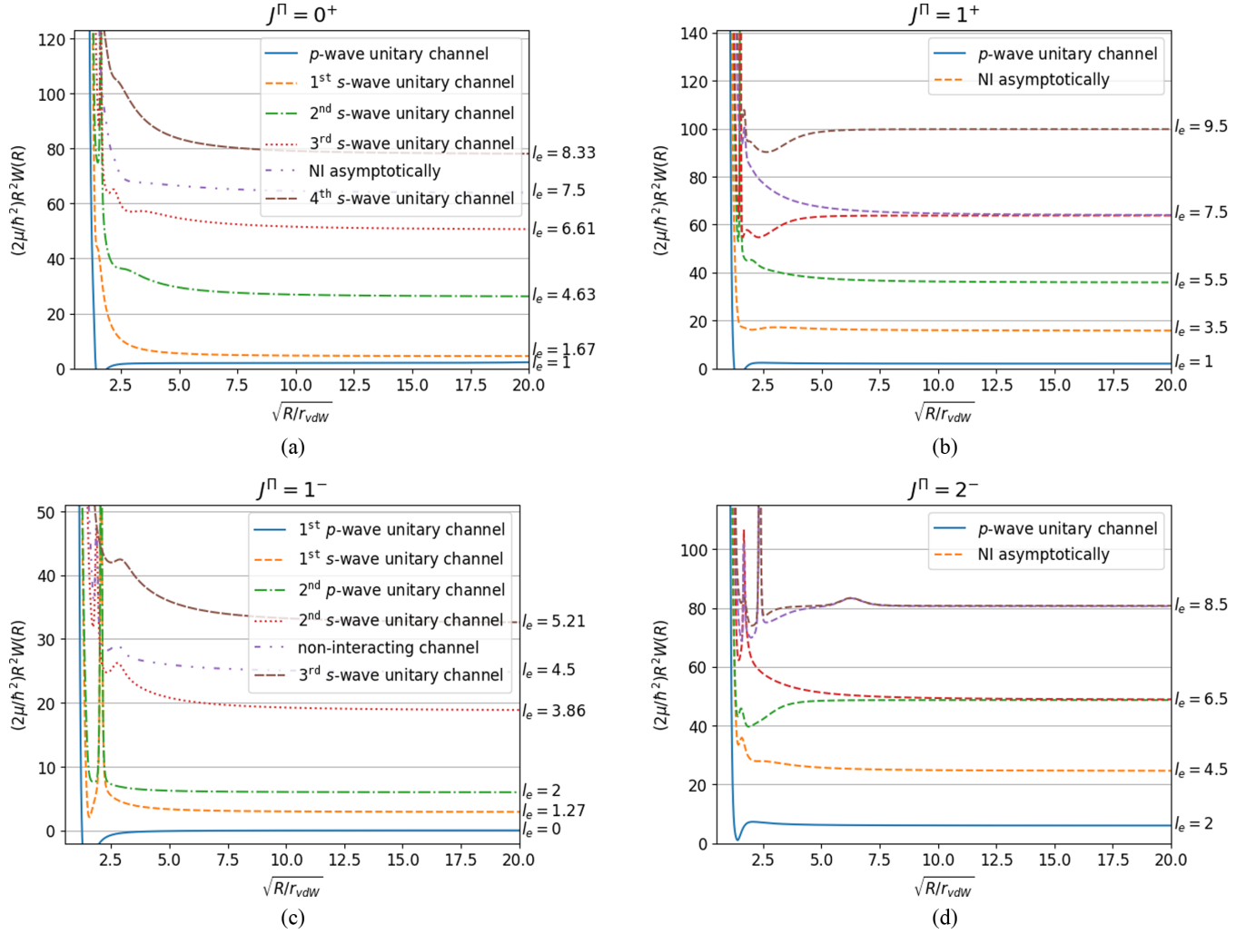
FIG. 2. Shown are the adiabatic potential curves for the first to sixth channels vs hyperradius for the (\downarrow\uparrow\uparrow) system. The interaction between the two fermions in the same spin state has been set at the p -wave unitary limit ( V_p \rightarrow \infty ), and the interactions between fermions in different spin states have also been set at the s -wave unitary limit ( a_s \rightarrow \infty ), for the various symmetries J^\Pi . (a), (b) The solid (blue) curve corresponds to the p -wave unitary channel, and the coefficient of 1/(2\mu R^2) is approximately 2. (c) The solid (blue) curve and dash-dot (green) curve show p -wave universal property, and their coefficients of 1/(2\mu R^2) are computed to have the values \approx 0.02 and \approx 6 , respectively. (d) The lowest adiabatic potential curve (solid curve) represents the p -wave unitary channel, and the asymptotic 1/(2\mu R^2) coefficient is calculated to have the value l_e(l_e + 1) \approx 6 .
