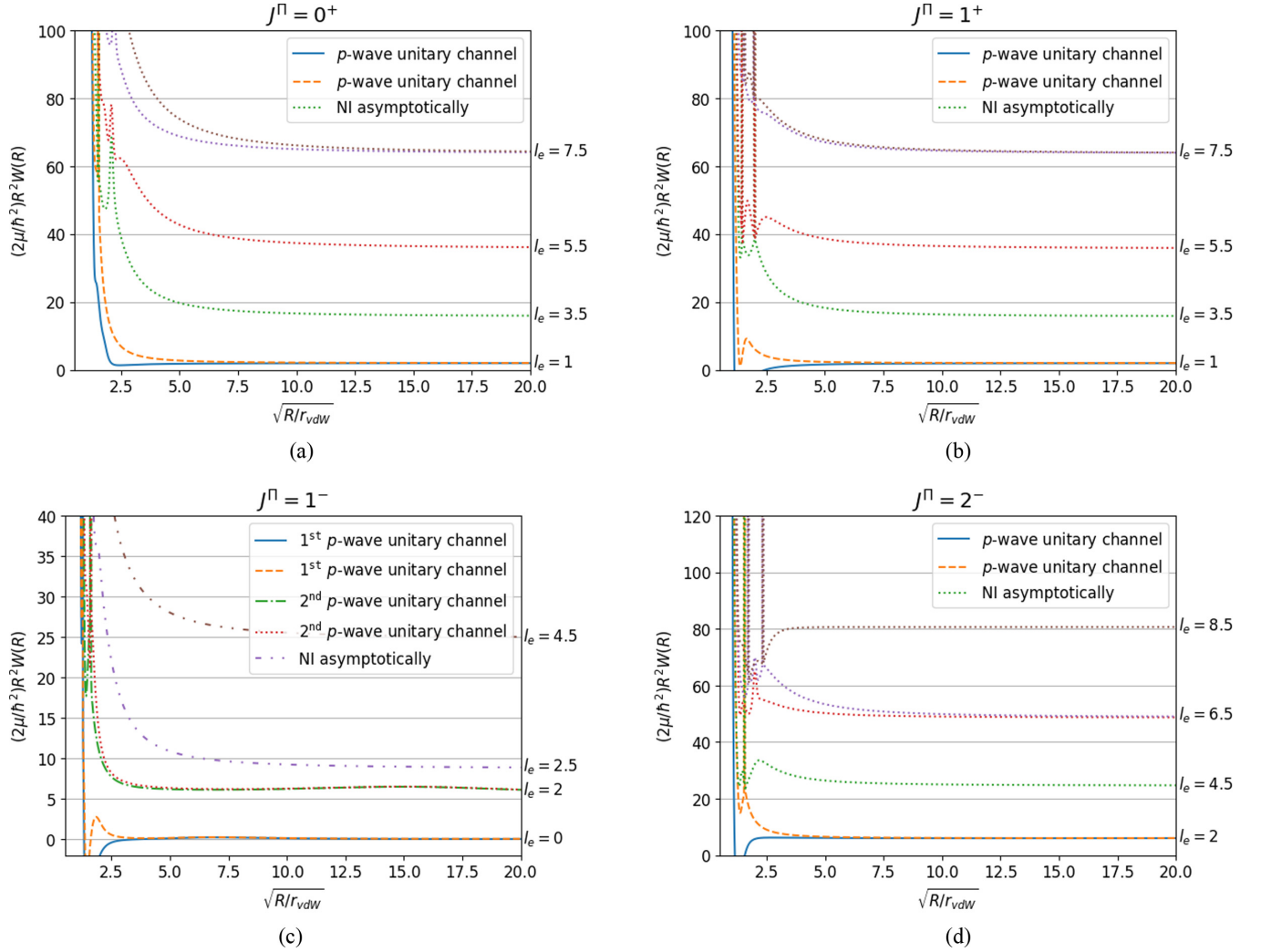
FIG. 4. The adiabatic potential curves for the first to sixth channels vs hyperradius for the fermions in the same and different spin state both at the p -wave unitary limit ( V_p \rightarrow \infty ) for the various symmetries J^\Pi . (a), (b) The solid (blue) and dashed (orange) curve corresponds to the p -wave degenerate unitary channel, and the coefficient of 1/(2\mu R^2) is approximately 2. (c) The solid (blue) curve and dashed (orange) curves show the first degenerate p -wave universal property, and their coefficients of 1/(2\mu R^2) are computed to have the values \approx 0.01 . The dash-dotted (green) curve and dotted (red) curve represent the second degenerate p -wave unitary channels with coefficients of 1/(2\mu R^2) close to 6. (d) The two lowest adiabatic potential curves (solid and dashed curves) represent the degenerate p -wave unitary channels, and the 1/(2\mu R^2) coefficient is calculated to have the value \approx 6 .
