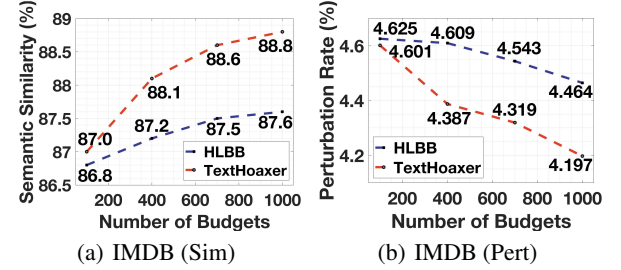
Figure 2: Performance comparison w.r.t. different budget limits between HLBB and TextHoaxer against WordLSTM.
