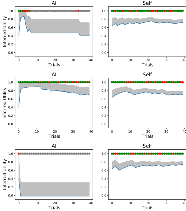
Figure 2: Illustrative results for the basic metacognitive bandit for three participants (rows) with inferred utilities for the AI arm (left column) and self arm (right column). The shaded region shows the posterior uncertainty associated with the inferred utility. Dots correspond to the rewards observed for each arm pull. The panels on the left show the human’s inferred utility of asking the AI for help. Gray dots correspond to the AI arm not being pulled, hence no reward was observed for those trials. Green and red dots corresponds to correct and incorrect responses respectively. The panels on the right show the human’s inferred utility of relying on own judgment and the associated reward sequence. The last row is an example of behavior that exemplifies the pattern often associated with algorithm aversion.
