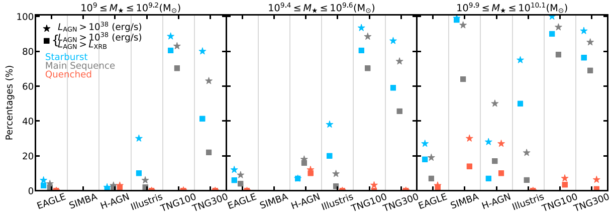
Figure 8. Percentages of galaxies at z = 0 with hard X-ray luminosity L_{\text{AGN}} > 10^{38} \text{ erg s}^{-1} (shown as stars) and percentages of those galaxies which have a brighter AGN than the galaxy-wide XRB population, i.e. L_{\text{AGN}} > L_{\text{XRB}} (shown as squares). We derive these percentages for different galaxy types colour coded as: starburst (blue), main sequence (grey) and quenched (red). While only a small fraction of quenched galaxies host an AGN in most of the simulations, the fraction among starburst and main-sequence is more important. Starburst galaxies are not always the galaxies hosting the largest number of AGN (see Horizon-AGN). The fraction of galaxies for which the AGN outshine the galaxy-wide XRB population is significantly lower for all galaxy types and simulations.
