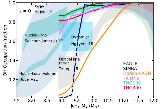
Figure 1. The BH OF for the local universe ( z = 0 ) predicted by the six simulations. Poisson error bars are shown as shaded regions, and are larger in more massive galaxies due to the presence of fewer galaxies. We show the fraction of SIMBA as a dashed line for M_\star < 10^{9.5} M_\odot , as only more massive galaxies are seeded. We include the current observational constraints on the BH OF of Nguyen et al. (2018) with dynamical mass measurement of BHs in a few nearby nucleated galaxies, and from Miller et al. (2015) and Trump et al. (2015), both derived from a sample of AGN in low-mass galaxies. While not being a constraint on the BH OF, we also report the galaxy nucleation fraction in the galaxy cluster Virgo (Sánchez-Janssen et al. 2019) and in the Local Volume (Hoyer et al. 2021).
