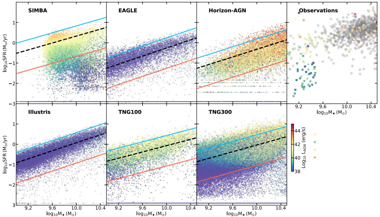
Figure 7. SFR– M_* diagram at z = 0 for the six cosmological simulations. Galaxies with SFR lower than 10^{-3} M_\odot/\text{yr} are set to this value. Galaxies are colour coded by the hard X-ray luminosity of their AGN. We set all AGN luminosity values lower than L_{\text{AGN}} = 10^{38} \text{ erg/s} (including inactive BHs) to the aforementioned value. We show the star-forming main-sequence of each simulation with a black dashed line. Starburst galaxies are located above the blue lines, and quiescent galaxies below the red ones. In the right-hand panel, we show several recent samples of galaxies from Mezcuza & Domínguez Sánchez (2020), Birchall et al. (2020), and Martín-Navarro, Shankar & Mezcuza (2021). Observed galaxies are colour coded (when possible, otherwise in grey) according to the luminosity of their AGN, as for the simulations. For a fair comparison, we have converted the AGN luminosity of several of these samples to hard (2–10 keV) X-ray luminosity.
