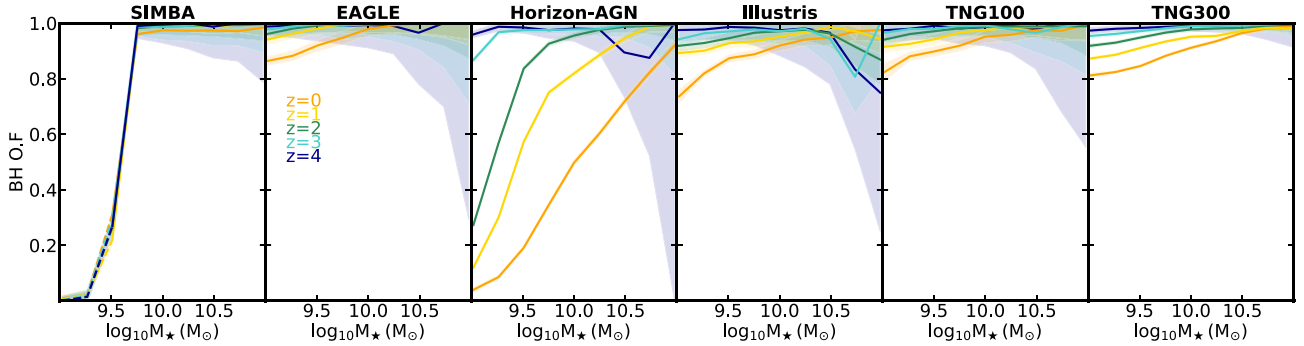
Figure 2. The BH OF at redshift z = 0-4 predicted by the all six simulations, over the range 10^9 M_\odot \leq M_\star \leq 10^{11} M_\odot (including both central and satellite galaxies). Shaded areas represent Poisson error bars. All the simulations have a higher BH OF at higher redshift, at fixed stellar mass. With time, the fraction drops in the low-mass galaxy regime. This is mainly due to a larger number of satellite galaxies that do not host a BH. The decrease is stronger in the Horizon-AGN simulation.
