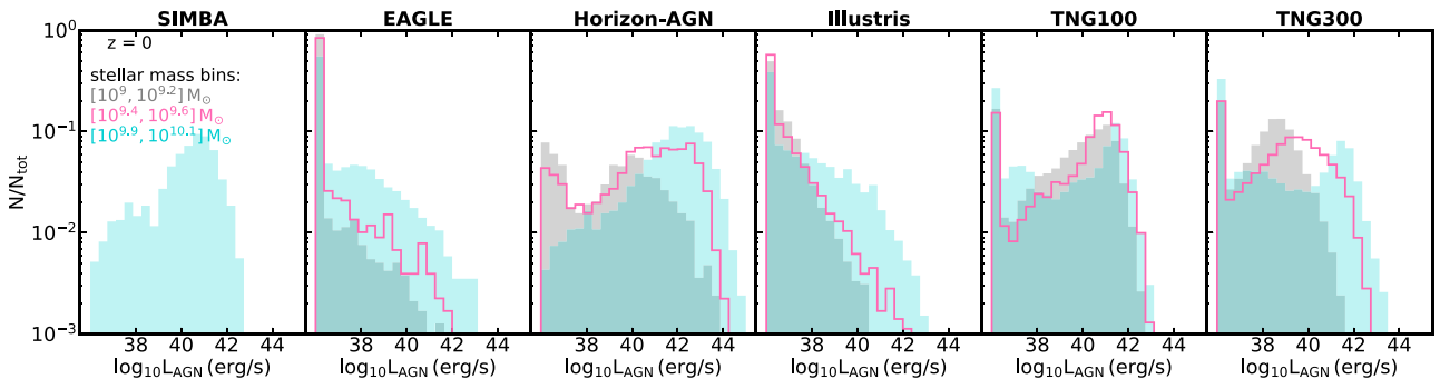
Figure B1. The normalized distribution of X-ray AGN luminosity at z = 0 galaxies with M_{\star} \sim 10^9 , \sim 10^{9.5} , \sim 10^{10} M_{\odot} for all the six simulations. For SIMBA, we do not display the BH population for M_{\star} < 10^{9.5} M_{\odot} since the simulation starts seeding BHs at the aforementioned value.
