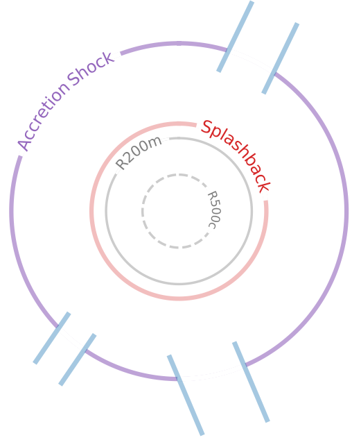
Figure 1. Illustration of the different cluster radii relevant to this work, denoted by colors and labelled by text. Radii are shown on linear axes, and are drawn to relative scales determined for the median SPT cluster mass and redshift — R_{500c} = 0.8 Mpc, R_{200m} = 1.6 Mpc, R_{sp} = 1.2R_{200m} = 1.9 Mpc, and R_{sh, acc} = 2.3R_{200m} = 3.7 Mpc. The estimate for the ratio R_{sp}/R_{200m} was taken from Shin et al. (2019), while R_{sh, acc}/R_{200m} was taken from Baxter et al. (2021). The blue lines show different filaments connected to the galaxy cluster. The accretion shock is expected to be weak/non-existent along filamentary directions. The splashback radius of the dark matter can be smaller than R_{200m} depending on the mass accretion rate of the cluster.
