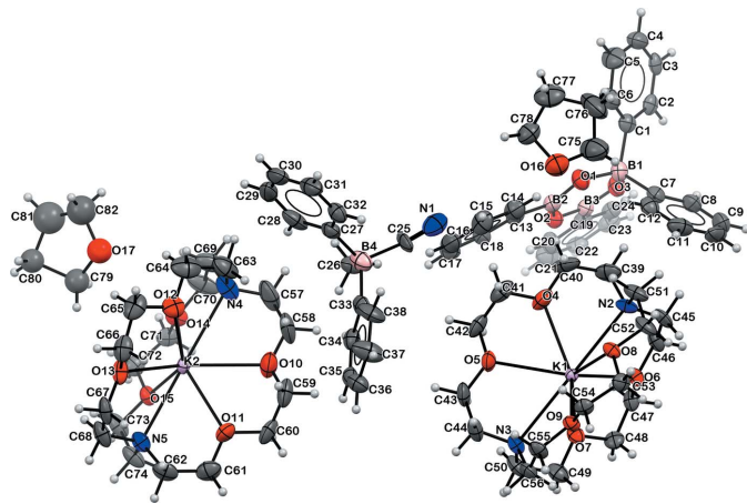
Figure 4 Displacement ellipsoid plot of 4 , [K(crypt)] 2 [B 3 (μ-O) 3 (C 6 H 5 ) 4 ][NCBPh 2 Me], drawn at the 50% probability level.
