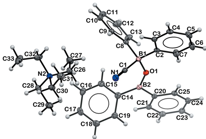
Figure 3 Displacement ellipsoid plot of 3 , [NEt 4 ][NCBPh 2 (μ-O)BPh 2 ], drawn at the 50% probability level.
