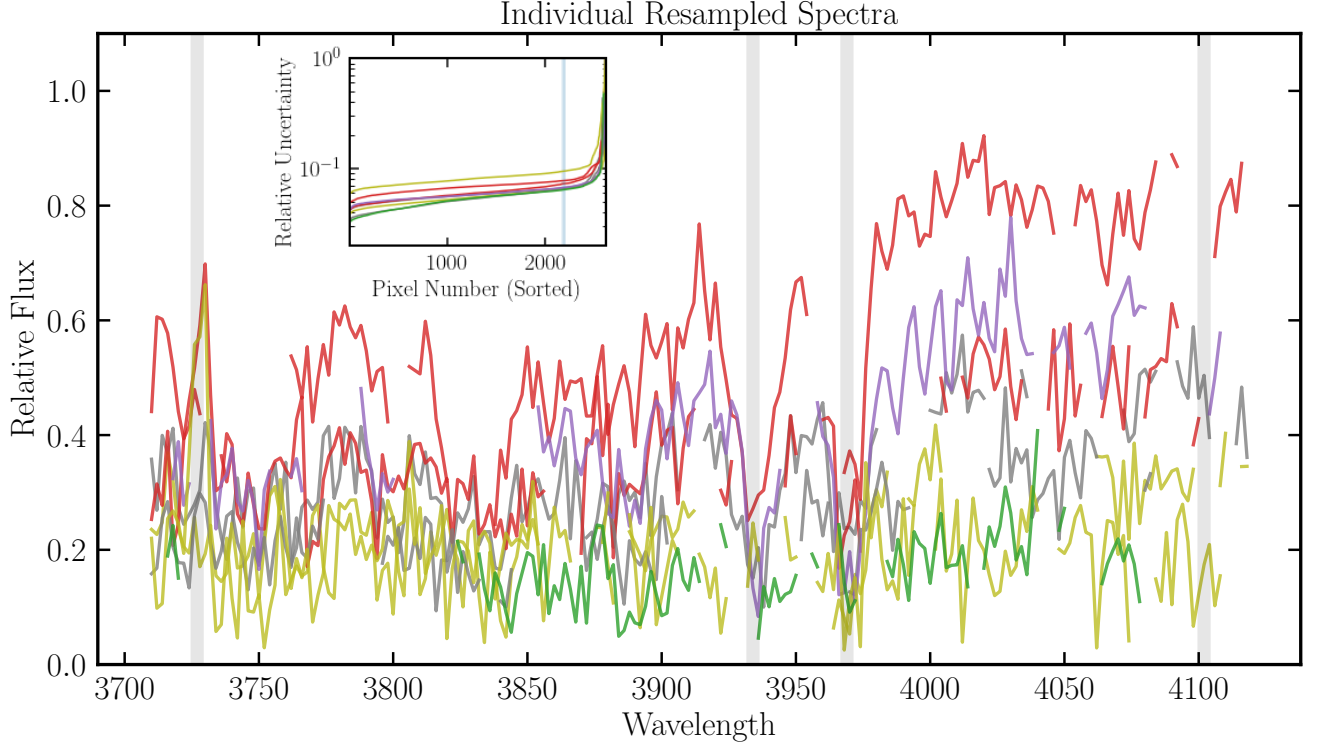
Figure 4. Noise-masked and resampled rest-frame spectra for all observed galaxies, prior to signal-to-noise, quiescent galaxy and stellar mass selection, in the cluster SPT-CL J0013-4906 at z=0.41 (colors represent spectra from different member galaxies). Shaded gray regions represent spectral features of interest in SED fitting (from left to right) — [OII] \lambda 3727, 3729\text{\AA} doublet, Ca II K&H \lambda 3934, 3968\text{\AA} and H\delta at 4102\text{\AA} . [OII] and 4000\text{\AA} break are used here to make quiescent galaxy cuts. (Inset) Relative sorted flux uncertainties per pixel for the same spectra in SPT-CL J0013-4906. The blue vertical lines denote the error threshold (84th percentile) above which spectral pixels are masked, followed by resampling.
