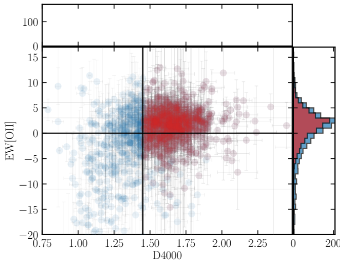
Figure 3. Distribution of equivalent width EW[OII] vs spectral index D4000 for sample galaxies (blue) and galaxies classified as quiescent in this work (red). EW[OII] vs D4000 is used here as an indicator for quiescent vs non-quiescent (actively star-forming, starburst or post-starburst) galaxies. Horizontal and vertical lines demarcating regions in the equivalent-width phase spaces are taken from Bruzual A. (1983) and Balogh et al. (1999) — quiescent galaxies have D4000 > 1.45 and no detection of an [OII] emission feature at > 2\sigma . We also test a more probabilistic cut for D4000 (i.e. D4000 > 1.45 at > 2\sigma ), which does not significantly impact our results.
