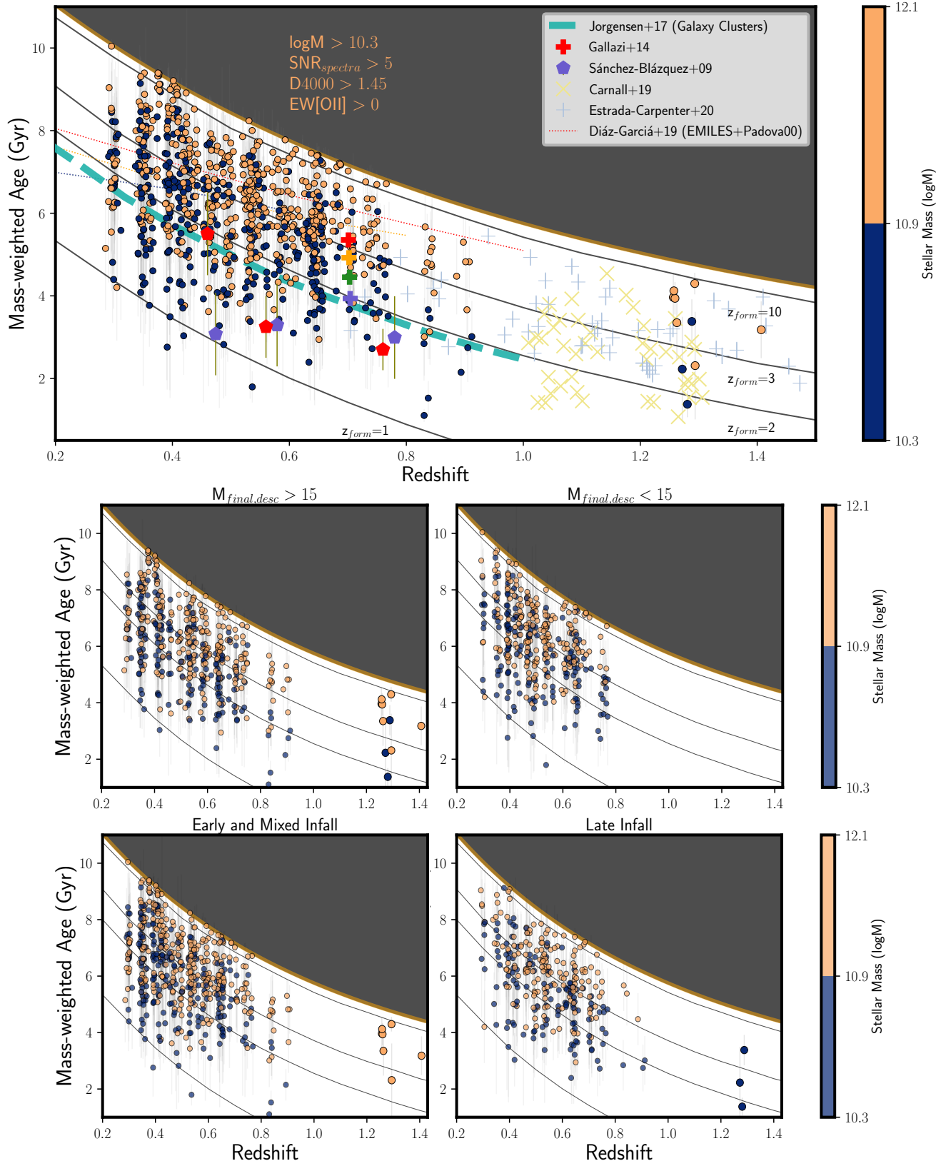
Figure 8. (Top) Mass-weighted Age (Gyr) as a function of observed redshift. The circle points represent ages of galaxies from this work, with blue (orange) points representing galaxies with low (high) stellar mass, as calculated via the SED fitting analysis. These measurements are compared to a wide range of literature on cluster galaxies and massive quenched galaxies in the field (see Section 6) e.g., Sánchez-Blázquez et al. (2009) and Gallazzi et al. (2014) measure ages for quiescent galaxies at 10 < \log M < 10.4 (purple) and \log M > 11.2 (red) (see Table 4). (Middle) Age vs redshift for galaxies in clusters with M_{\text{final,desc}} > 15 (left) and M_{\text{final,desc}} < 15 (right). (Bottom) Age vs redshift for galaxies with early and mixed infall (left) and late infall (right), as measured from their phase-space location in velocity-radius space. Black lines indicate the age of simple stellar populations (SSPs) with different formation redshifts as labeled in the top panel.
