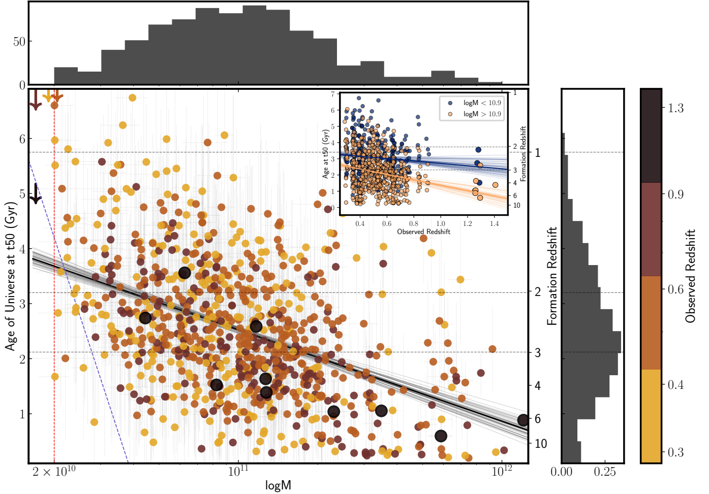
Figure 11. Age of Universe at which the galaxy has formed 50% of its mass (corresponding to t_{50} , in Gyr) vs \log M for quiescent galaxies considered in this work. Color at each point denotes the observed redshift, with orange points at z \sim 0.3 and large black points at z \sim 1.3 , the highest redshift galaxies in the sample. Best-fit age-mass relation is plotted in black, with grey lines sampling 50 lines from randomly sampled combinations of slopes and intercepts in the range of best-fit values and 1\sigma uncertainties. Downward arrows correspond to the maximum age of the Universe allowed for the median redshift in each bin — 5.1 Gyr at z = 1.28 , and 9.1 Gyr at z = 0.37 . Overplotted are the fixed mass cut considered in this work (dotted red line). We also show a fixed detectability (or SNR) cut for the lowest mass galaxies near the B16 survey detection limit (in dotted blue), with the slope of the line equal to the best-fit age-(L/M) relation; see Section 6.2.1 for details. (Inset) Age of Universe at t_{50} (Gyr) vs Observed redshift, for galaxies studied in this work, split by stellar mass.
