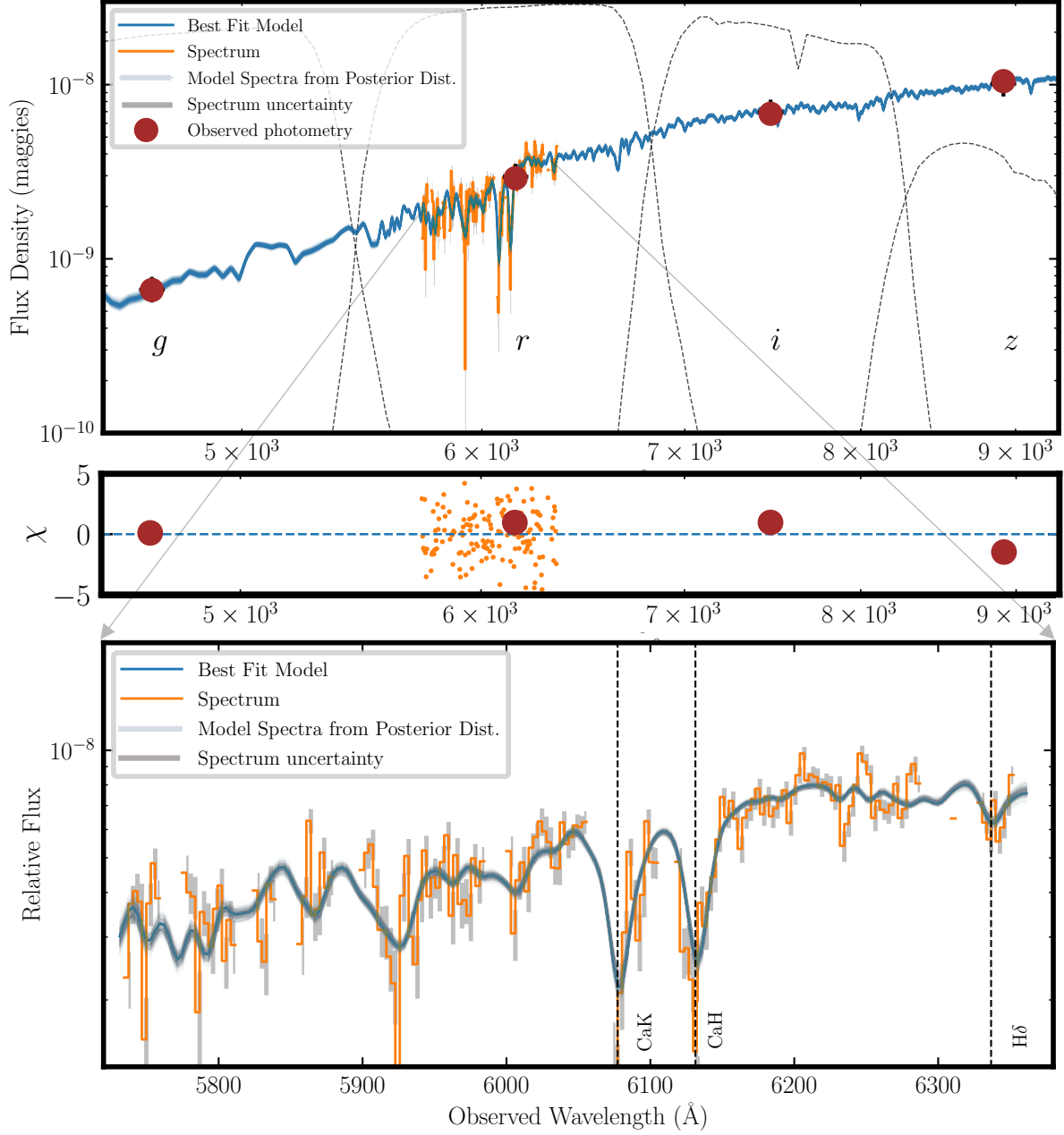
Figure 5. (Top) SED of a massive quiescent member galaxy of SPT-CL J2335-4544 at z = 0.55 , shown as flux density (maggies, Jy/3631) vs. observed wavelength ( \text{\AA} ). Model fits (blue) to photometry (brown) and spectrum (orange) are shown. (Middle) Residual ( \chi ) values for spectrum and photometry. Photometric data considered here is precise (uncertainties < 0.03 mag). (Bottom) Zoomed-in version of the spectrum, uncertainty and best-fit model.
