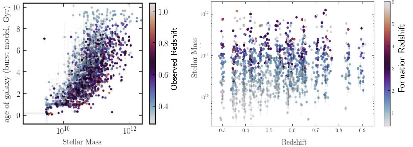
Figure 22. (Left) Ages (in Gyr) as a function of stellar mass (in M_{\odot} ) for a single burst fixed metallicity model-based (Model B), with color indicating observed redshifts. (Right) Stellar Mass vs redshift for the low- z member galaxies in our sample, corresponding to Model B. Colors correspond to formation redshifts, where more massive galaxies ( \log M > 11 ) were formed at z > 3 .
