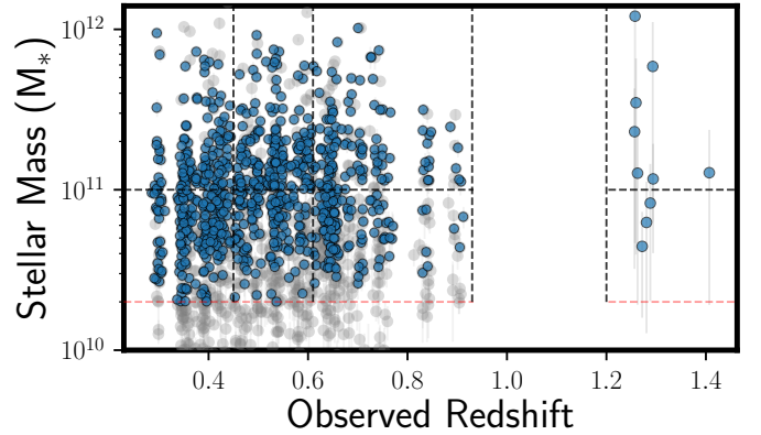
Figure 7. Stellar mass ( M_{*} ) as a function of redshift for member galaxies in the SPT-GMOS survey for clusters at 0.3 < z < 0.9 , as characterized by an SED fit to individual galaxies via a delayed-tau SFH model (i.e. Model A, grey points). We exclude a small fraction of galaxies with masses < 2 \times 10^{10} M_{\odot} ( \log M < 10.3 ) to create a uniform lower limit on the galaxy masses and median mass per bin; the quiescent galaxies considered in this sample are marked with blue points. The dotted lines mark the stellar mass and redshift bins used in this work.
