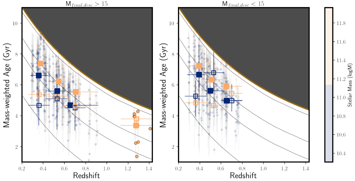
Figure 19. Same as top panels of Figure 9, but hollow squares signifying stacked spectra mass-weighted ages where stacking is performed using the alternate method described here.
