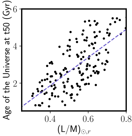
Figure 13. Age of Universe at which the galaxy has formed 50% of its mass (corresponding to t_{50} , in Gyr) vs inverse of mass-to-light ratio ( L/M ) (in solar units) for D_{4000} > 1.45 quiescent galaxies drawn from model SEDs. The best-fit relation is plotted as a dotted blue line.
