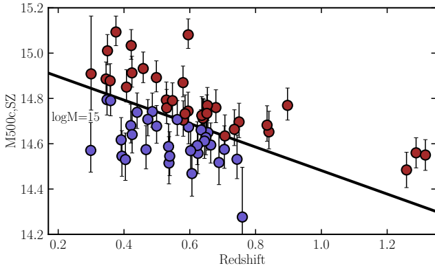
Figure 2. \log(M_{500c,SZ}/M_{\odot}) vs redshift for 64 clusters in the High- z and Low- z samples. The black line demarcates the evolutionary path of galaxy clusters to final cluster mass at redshift 0 of \log(M_{500c,SZ,z=0}/M_{\odot}) = 15 . The cluster sample is divided into two groups based on this demarcation, to facilitate a descendant-antecedent analysis of member galaxies (Fakhouri et al. 2010) — blue (red) points are clusters with final descendant cluster mass of \log(M_{500c,SZ,z=0}/M_{\odot}) < 15 ( > 15 ).
