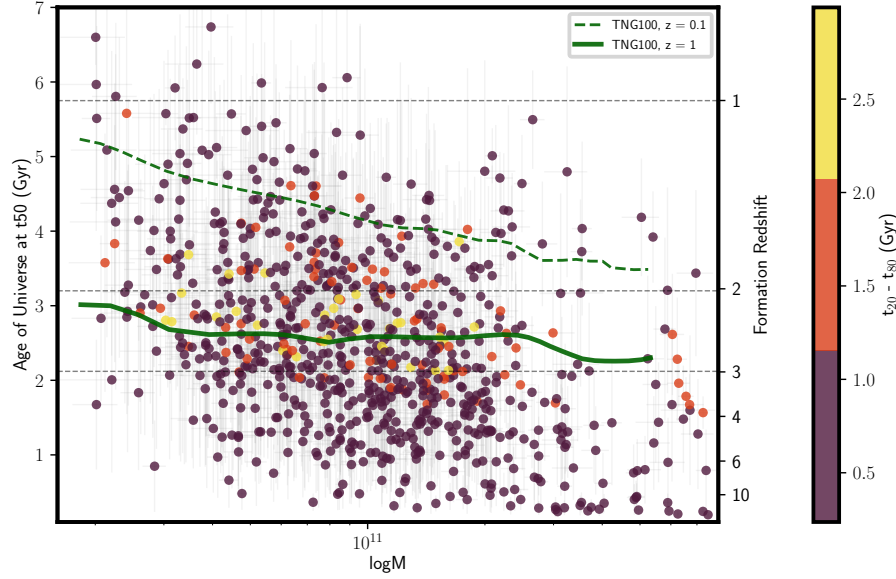
Figure 16. Same as Figure 11, with points color-coded to represent star formation timescale, as calculated with the parameter t_{20}-t_{80} (Gyr). Dark green dotted and solid lines represent ages of Universe at formation times vs \log(M) from the TNG100 simulations and redshifts 0.1 and 1 respectively, as seen in Figure 8 of Carnall et al. 2019b . The most massive galaxies have mostly formed before z > 2 , while the lowest-mass galaxies have formation redshifts of z < 3 . While the most massive galaxies have formed stars in the shortest time-scales, we observe that the most extended star-formation is shown by galaxies at formation redshifts between 1.5-3.5.
