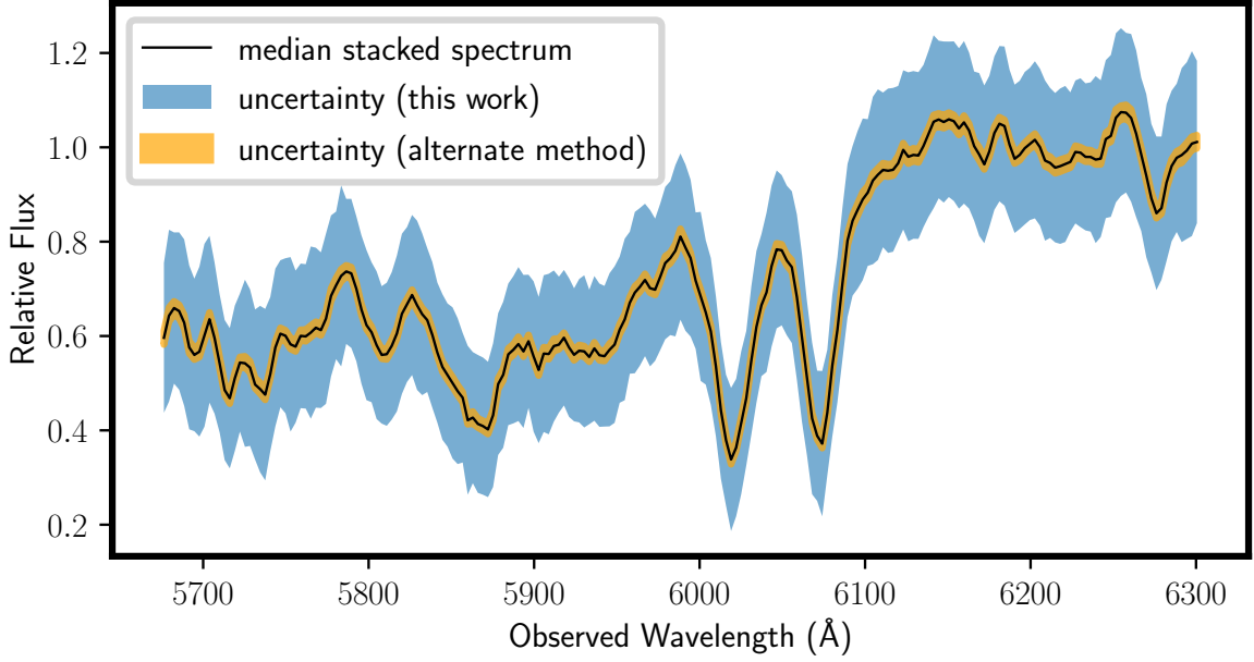
Figure 21. Stacked spectrum generated for galaxies in the \log(M_{500c, SZ, z=0}/M_{\odot}) > 15 , \log M > 10.90 and z = 0.53 bin in our sample. The median stacked spectrum is plotted in black, while the stacked spectrum uncertainty considered in this work is plotted in blue. Orange denotes the uncertainty derived from the alternate stacking method, which — as we argue in this section — biases age calculations and may underestimate uncertainty.
