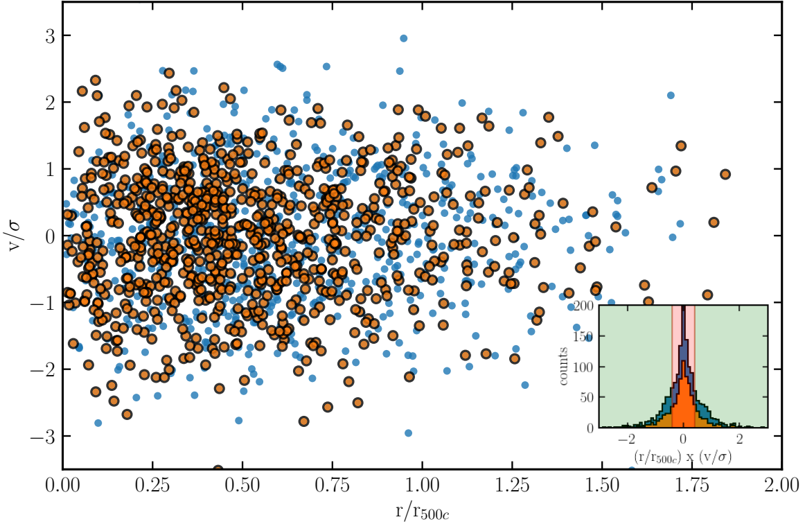
Figure 1. Normalized proper velocity vs. normalized distance of member galaxies in the sample from the nominal cluster SZ center. Velocities are normalized to the velocity dispersion of the galaxy cluster. Orange points correspond to quiescent galaxies in the sample, while blue points represent non-quiescent galaxies. (Inset) A histogram of the distribution of phase-space location (or proxy for ‘infall time’) for all galaxies (blue) and quiescent galaxies (orange), defined as p = r_{\text{projected}}/r_{500c} \times v_{\text{peculiar}}/\sigma_v . The shaded red region corresponds to galaxies in the ‘early+mixed infall’ subpopulation i.e. p < 0.4 .
