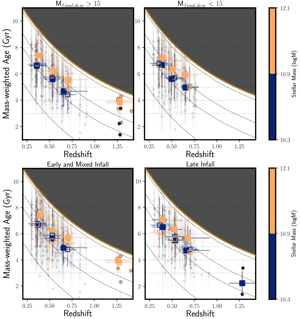
Figure 9. (Top) Mass-weighted Age (Gyr) as a function of observed redshift (same as Figure 8), to illustrate aggregate and stacked spectra properties of each subpopulation considered in this work. Solid filled squares correspond to median ages per redshift and stellar mass bin (with standard deviation of the ages represented by the error bars). Non-filled squares correspond to stacked spectra ages.
