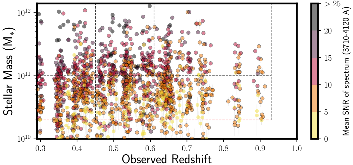
Figure 23. Same as Figure 7, with average signal-to-noise ratio of the observed spectrum coded with color for each galaxy spectrum in the low- z cluster sample ( 0.3 < z < 0.9 ), where we employ an SNR cut. Points with black borders are the 827 galaxies considered in this study from the low- z cluster sample. The highest SNR spectra were observed from the higher mass galaxies in the sample.
