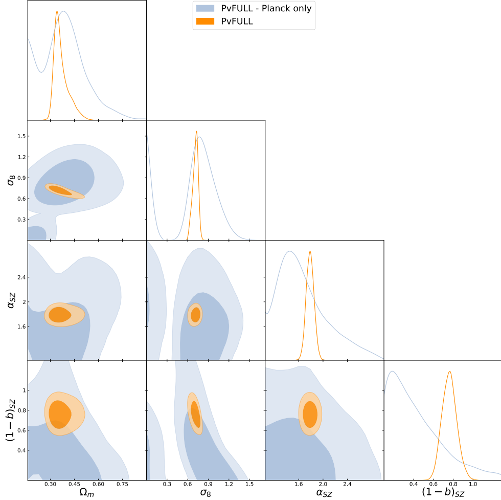
Figure 6. We show the one-dimensional and two-dimensional probability distributions for the cosmological ( \Omega_m , \sigma_8 ) and Planck scaling relation ( \alpha_{SZ} , (1-b)_{SZ} ) parameters. The contours represent the 68% and 95% CL. We compare results for the complete Planck analysis (Planck clusters + BAO + BBN + external scaling relation calibrations assuming self-similar redshift evolution) in orange, with results obtained considering only Planck clusters (light blue).
