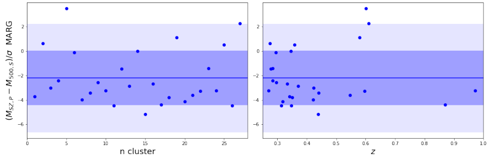
Figure 10. We show the distribution of mass differences for the 27 clusters in common between Planck and SPT-SZ cosmological catalogs, as a function of the cluster number (left) and redshift (right). For the Planck clusters, we consider M_{SZ} estimates. For the SPT-SZ clusters we consider the mass estimates marginalised over cosmological and scaling relation parameters. The shaded areas represent the 1\sigma and 2\sigma intervals of the distribution.
