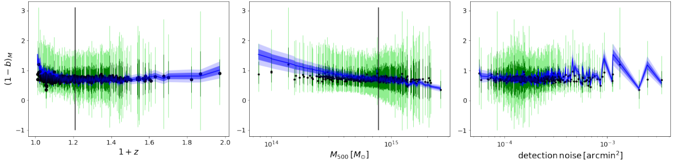
Figure 4. Mass bias evaluated from the Monte-Carlo extracted masses M_{500} , (1-b)_M = M_{\text{SZ}}/M_{500} . We show the mass bias as a function of redshift (left panel), M_{500} (middle panel) and detection noise (right panel): we report the best-fit (black points) with 68% (dark green) and 95% (light green) error bars. The blue shaded area represents the trend and the 68% and 95% CL obtained when fitting Eq. 22, following results in Table 6. The black vertical lines show the values of z_* and M_* .
