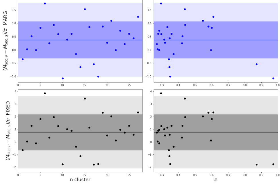
Figure 9. We show the distribution of mass differences for the 27 clusters in common between Planck and SPT-SZ cosmological catalogs, as a function of the cluster number (left) and redshift (right). We compare the results when considering the mass estimates marginalised over cosmological and scaling relation parameters (in blue, top panels) and obtained with fixed cosmological and scaling relation parameters (in black, bottom panels). The shaded areas represent the 1\sigma and 2\sigma intervals of the distribution.
