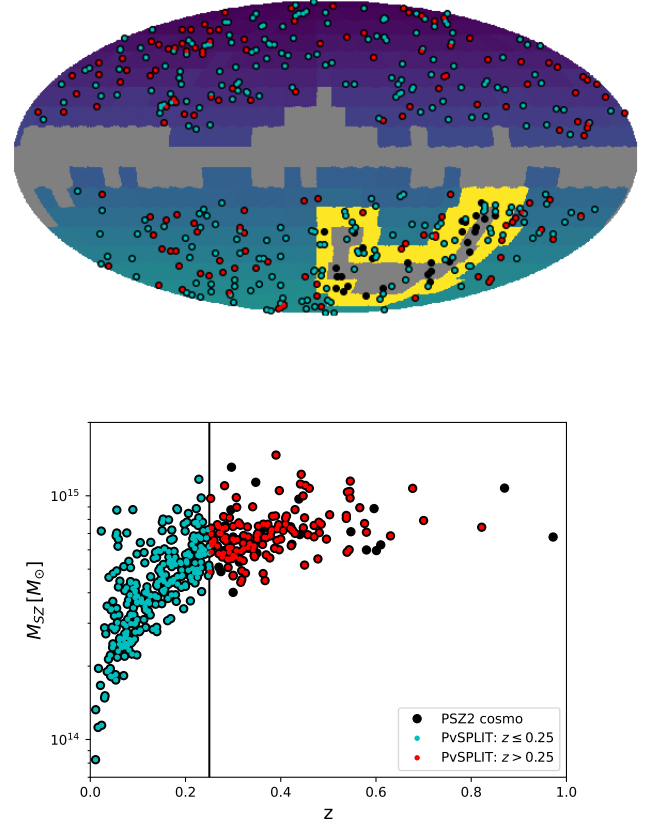
Figure 1. Upper panel. Map of Planck patches in galactic coordinates. In grey we show the removed patches, due to the Planck galactic mask and the fully overlapped area with SPT observations. In yellow we highlight the 35 partly overlapping patches between Planck and SPT. Upper and lower panel. Comparison between the PSZ2 cosmo catalog (black points), with the PvSPLIT catalog. In the upper panel, we show how the clusters are distributed in the sky. In the lower panel, we show the mass-redshift distribution, considering M_{SZ} mass from Planck Collaboration et al. (2016b). The cyan points are the clusters considered in the z \leq 0.25 part of the PvSPLIT likelihood. The red points are the clusters considered in the z > 0.25 PvSPLIT likelihood.
