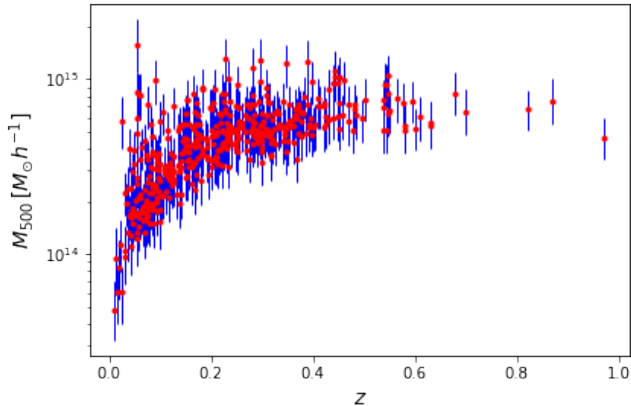
Figure 3. Cluster masses for the Planck cosmological sample, evaluated with a Monte-Carlo extraction approach. We show the best-fit value (red points) and the 68% c.i. error bars (in blue).
