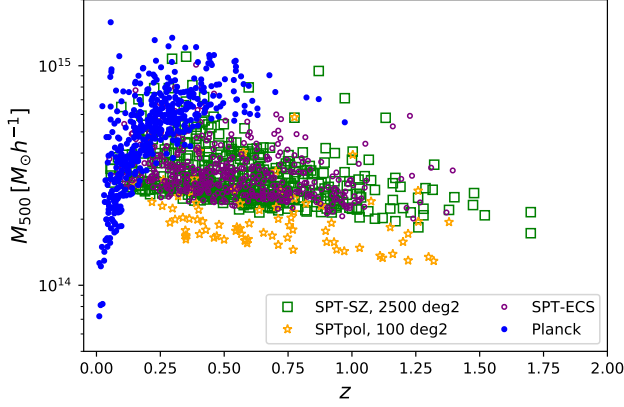
Figure 5. Evaluation of cluster masses, for each cluster in the Planck cosmological cluster sample (blue points), for fixed values of cosmological and scaling relation parameters. We report also the SPT cluster masses from the SPT-SZ 2500 deg 2 catalog (green squares), from the SPTpol 100 deg 2 catalog (yellow stars) and from the SPTpol Extended cluster catalog (purple circles).
