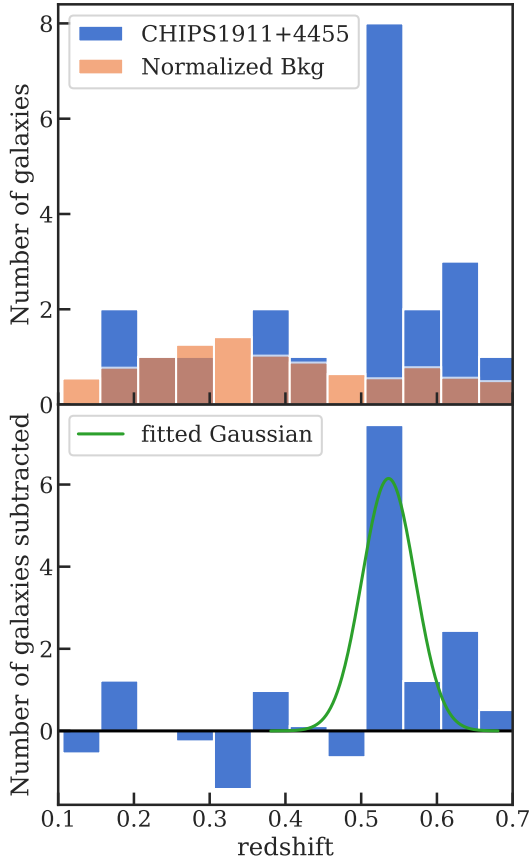
FIG. 9.— Top: The blue histogram shows the redshift distribution of all the galaxies within one arcmin of CHIPS1911+4455. The orange histogram shows the the renormalized distribution of background galaxies. Bottom: The background-subtracted histogram is shown in blue. The green solid line shows the fixed-width Gaussian fit between the peak and the two neighboring bins to estimate the richness. The significance of the redshift peak at z = 0.53 strongly suggests the presence of a galaxy cluster.
