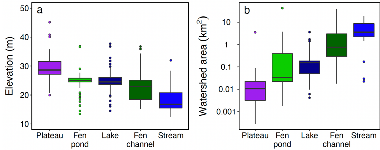
Figure S1. Distributions of watershed elevation and area by aquatic environment type.
