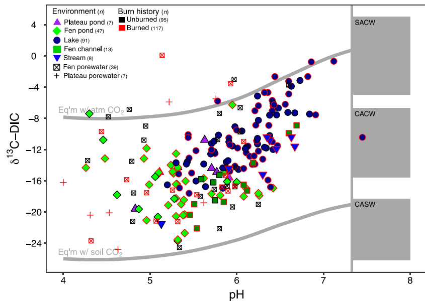
Figure 3. pH and the composition of stable dissolved inorganic carbon isotopes ( \delta^{13}\text{C-DIC} ) in aquatic environments within the Yukon Kuskokwim Delta (five surface water, two pore water). Reference lines depict theoretical end-member values for equilibrium reactions with atmospheric and biotic \text{CO}_2 , which—up to \text{pH} \sim 7.3 for these samples—have a greater effect on \delta^{13}\text{C-DIC} values compared with kinetic isotope fractionation effects from mineral weathering reactions. Proximity to gray areas ( \text{pH} > 7.3 ) reflects greater contributions to DIC from \text{H}_2\text{SO}_4 carbonate weathering (SACW), \text{H}_2\text{CO}_3 carbonate weathering (CACW), or \text{H}_2\text{CO}_3 silicate weathering (CASW) (Section 2.3).
