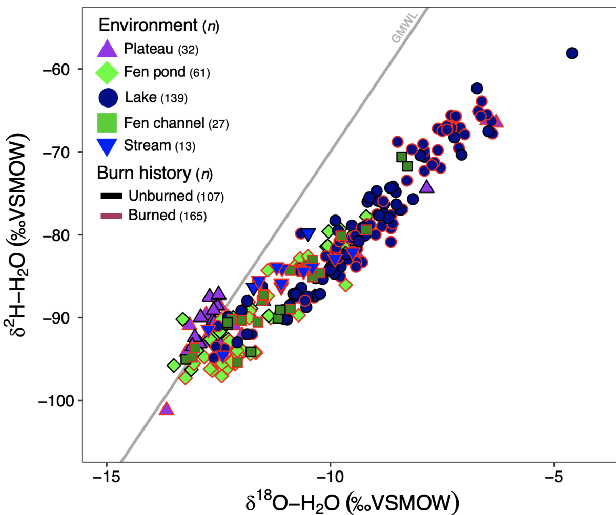
Figure S2. The stable isotopic composition of surface waters among the five aquatic environments in the Yukon-Kuskokwim Delta. GMWL = global meteoric water line.
