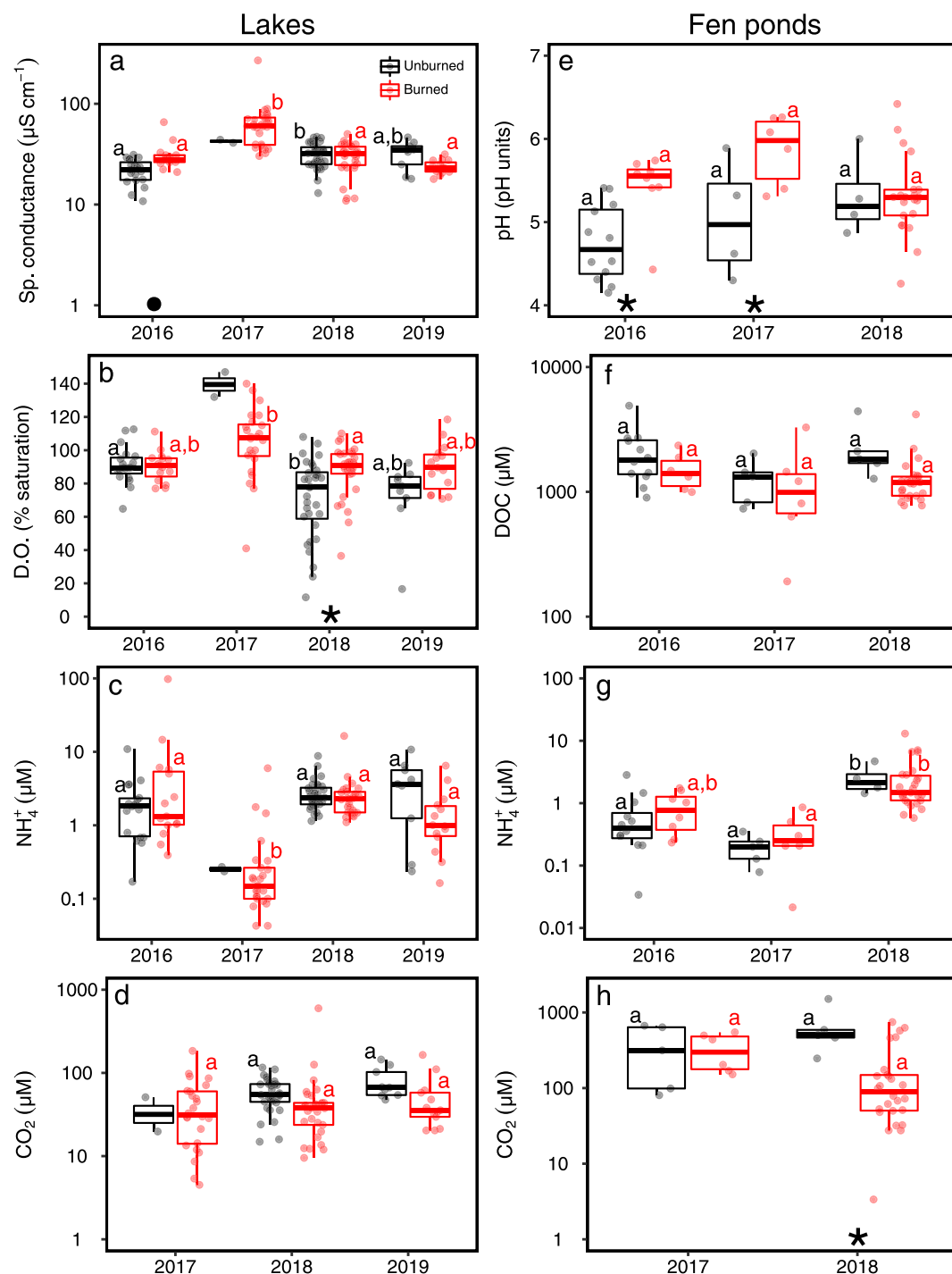
Figure 7. Surface water chemistry in lakes (a–d) and fen ponds (e–h). Considering sampling year within unburned and burned watersheds separately, boxes with different letters reflect significantly different mean values (e.g., specific conductance lakes within burned watersheds during 2017 vs. other years), as determined by perMANOVA (Section 2.5). Note: Letters above boxes are color-coded by burn history. Along the x-axis, * and • reflect statistically significant ( p < 0.05 ) and marginal ( 0.05 < p \leq 0.1 ) differences between unburned and burned sites within the corresponding aquatic environment (e.g., pH within burned vs. unburned fen ponds in 2016 and 2017). Horizontal line within each box represents the median. Horizontal lines below and above the median represent the first and third quantiles, respectively. Lower and upper whiskers extend from the first or third quantile to the smallest or greatest value, respectively, to no more than 1.5 times the inter-quantile range. All values, including outliers beyond the whiskers, are shown as individual points.
