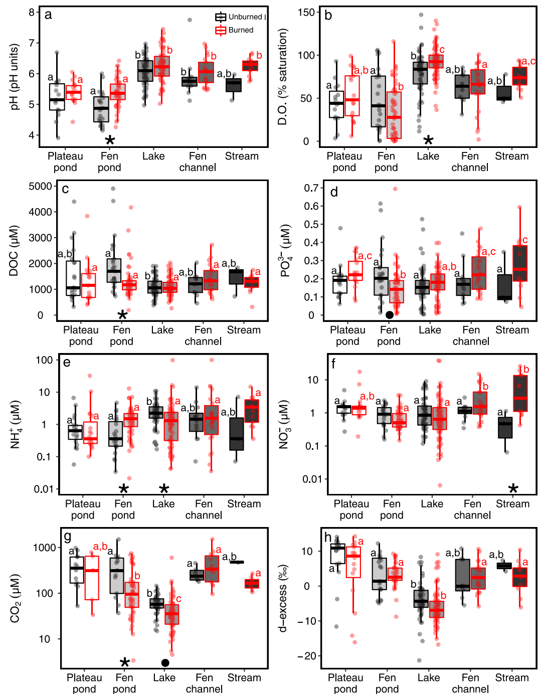
Figure 2. Surface water quality (a–b) and concentrations of dissolved organic carbon (c), nutrients (d–f), and CO 2 (g), and d-excess (h) in the five aquatic environments. Each site type is shaded differently, to help visualize and differentiate. Considering aquatic environments within unburned and burned watersheds separately, boxes with different letters reflect significantly different mean values (e.g., pH in fen ponds and lakes within burned watersheds), as determined by permANOVA (Section 2.5). Note: Letters above boxes are color-coded by burn history. Along the x-axis, * and • reflect statistically significant ( p < 0.05 ) and marginal ( 0.05 < p \leq 0.1 ) differences between unburned and burned sites within the corresponding aquatic environment (e.g., D.O.% within burned vs. unburned lakes). Horizontal line within each box represents the median. Horizontal lines below and above the median represent the first and third quartiles, respectively. Lower and upper whiskers extend from the first or third quartile to the smallest or greatest value, respectively, to no more than 1.5 times the inter-quartile range. All values, including outliers beyond the whiskers, are shown as individual points.
