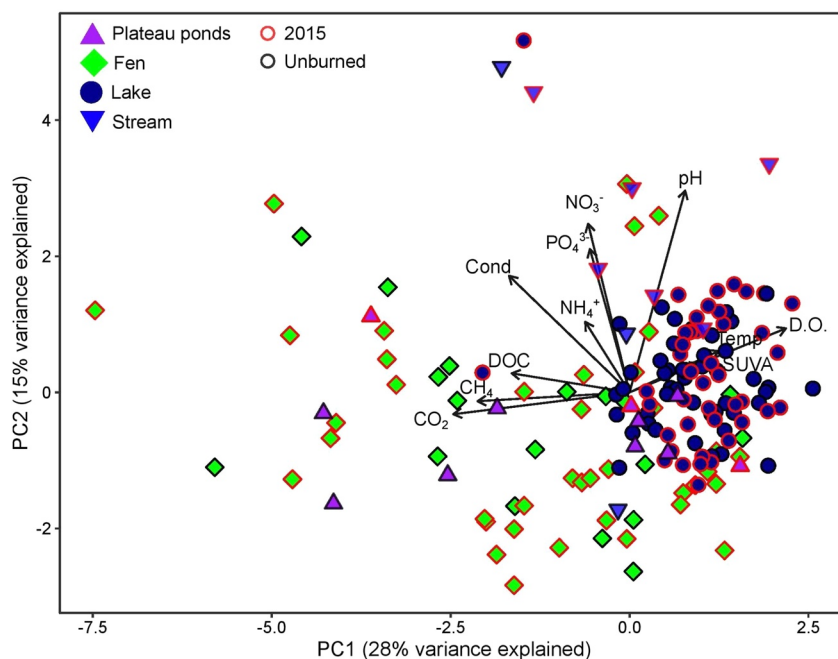
Figure 5. Principal component analysis of surface water geochemical variables for all landscape types. The shapes distinguish between plateau ponds, lakes, fens, and streams, while the border color represents control or burned in 2015. All vectors were multiplied by 5 to improve visibility.
