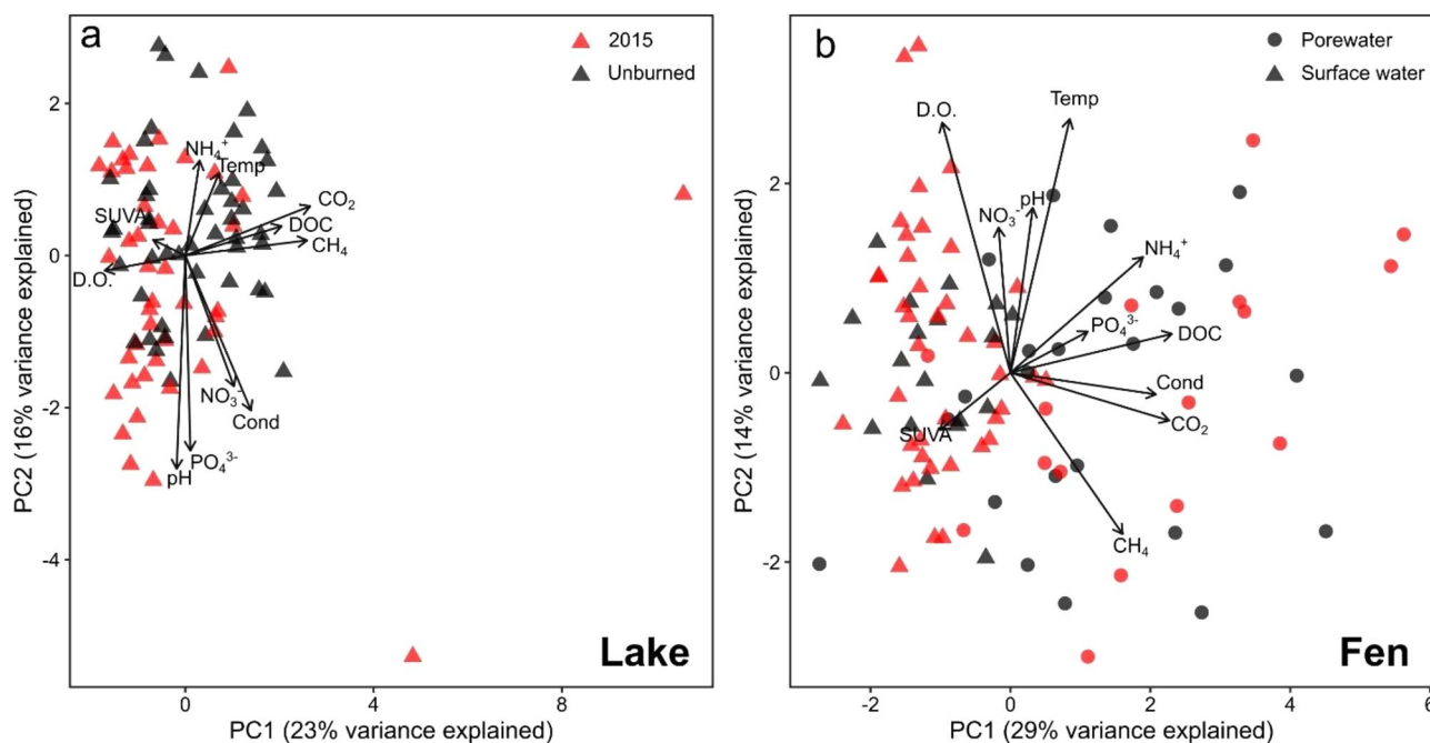
Figure 6. Principal component analysis of geochemical variables for (a) surface water samples from lakes and (b) both surface water and pore water samples from fens. Colors denote burn status (a and b) while shape distinguishes between pore water and surface water samples (b only). All vectors were multiplied by 5 to improve visibility.
