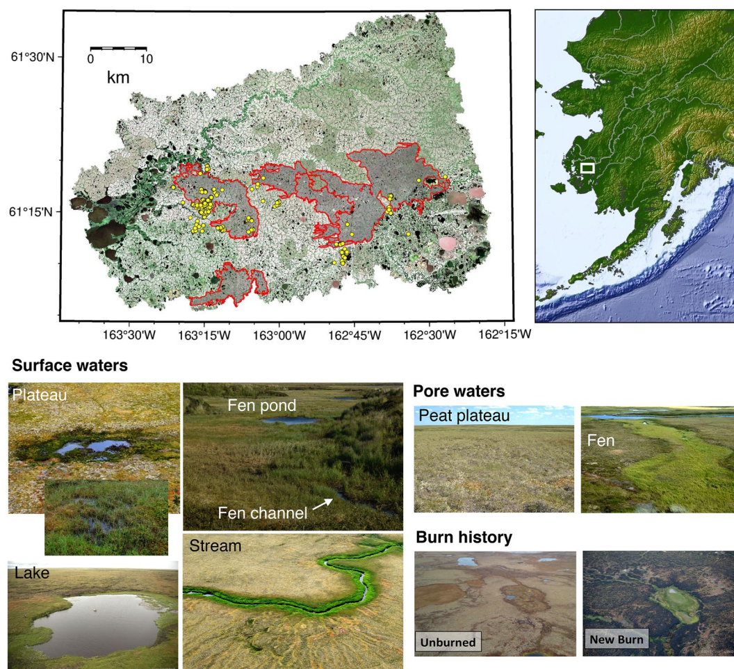
Figure 1. Top left: map of sampling sites (yellow points) within the study area. Red polygons outline perimeters of wildfires during 2015. Map created using Generic Mapping Tools (Wessel et al., 2019). Top right: location of study area within Alaska (white box). Terrain relief data obtained from Tozer et al. (2019). Bottom: aquatic environments within the Yukon-Kuskokwim Delta that were sampled for (a) surface waters and (b) pore waters across terrain that was (c) unburned or burned in 2015. Photographs are in true color and all were made by Chris Linder Photography.
