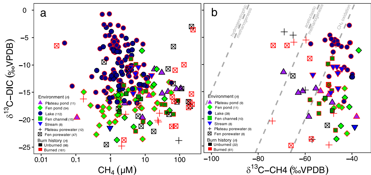
Figure 4. Stable isotopic composition of dissolved inorganic carbon ( \delta^{13}\text{C-DIC} ) as a function of (a) \text{CH}_4 concentration and (b) the stable isotopic composition of \text{CH}_4 ( \delta^{13}\text{C-CH}_4 ) in surface and pore waters of the Yukon-Kuskokwim Delta. Burn history depicts sites associated with wildfire. Equilibrium fractionation end-members (dotted lines) for methanogenic pathways and methanotrophy after Campeau et al. (2018).
