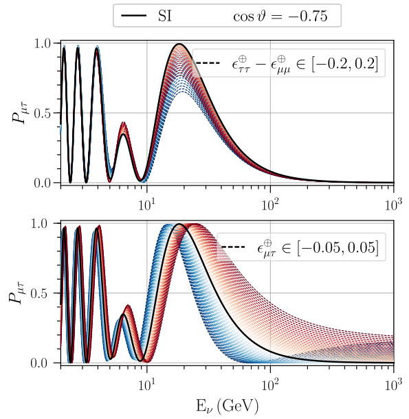
Figure 2: Examples of oscillation probabilities at different NSI hypotheses. Each panel shows P_{\mu\tau} for different positive (in red) and negative (in blue) values of the individual NSI parameter together with the standard interaction oscillations (SI) case in black.
