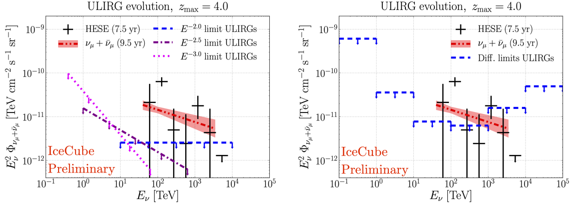
Figure 2: Upper limits (90% CL) on the contribution of the ULIRG source population up to a redshift z_{\text{max}} = 4.0 to the diffuse IceCube observations (black data points and red band). Left: Integral limits are shown for unbroken E^{-2.0} (dashed blue line), E^{-2.5} (dash-dotted dark magenta line), and E^{-3.0} (dotted light magenta line) power-law spectra, within the respective 90% central energy ranges that contribute to the upper limits. Right: Quasi-differential limits (dashed blue lines) are obtained by computing the E^{-2.0} limit in each bin of energy decade.
