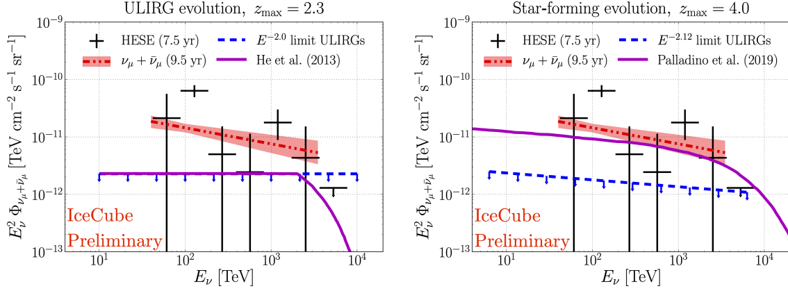
Figure 3: Comparison of our ULIRG upper limits (90% CL; dashed blue lines) to two model predictions (full magenta lines). Left: Comparison with the model of He et al. [9], where for the upper limit we assume an ULIRG source evolution integrated up to a redshift z_{\max} = 2.3 . Right: Comparison with the model of Palladino et al. [10], where for the upper limit we assume a source evolution according to the star-formation rate integrated up to a redshift z_{\max} = 4.0 .
