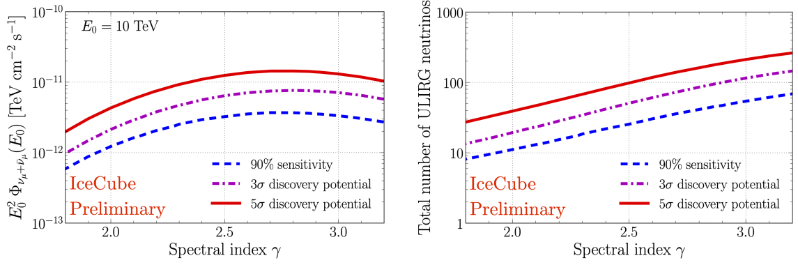
Figure 1: Sensitivity, 3\sigma , and 5\sigma discovery potentials for an unbroken E^{-\gamma} power-law spectrum. Left: Shown in terms of the flux at the normalization energy E_0 = 10 TeV. Right: Shown in terms of the total number of ULIRG neutrinos.
